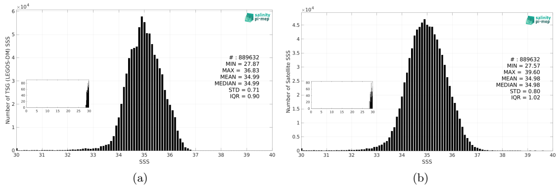
Figure 3: Histograms of SSS from TSG (LEGOS-DM) (a) and SMAP SSS L2 v6 (RSS) (b) considering all match-up pairs per bins of 0.1 over the Tropical Pacific Ocean Pi-MEP region and for the full satellite product period.
