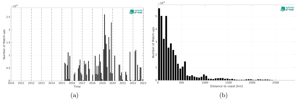
Figure 2: Number of match-ups between TSG (GOSUD-Research-vessel) and SMAP SSS L2 v6 (RSS) SSS as a function of time (a) and as function of the distance to coast (b) over the Tropical Pacific Ocean Pi-MEP region and for the full satellite product period.
