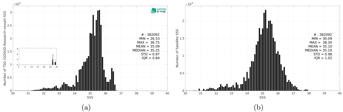
Figure 3: Histograms of SSS from TSG (GOSUD-Research-vessel) (a) and SMAP SSS L2 v6 (RSS) (b) considering all match-up pairs per bins of 0.1 over the Tropical Pacific Ocean Pi-MEP region and for the full satellite product period.
