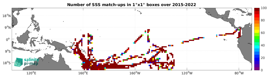
Figure 5: Number of SSS match-ups between TSG (GOSUD-Research-vessel) SSS and the SMAP SSS L2 v6 (RSS) SSS product for the Tropical Pacific Ocean Pi-MEP region over 1^\circ \times 1^\circ boxes and for the full satellite product period.
