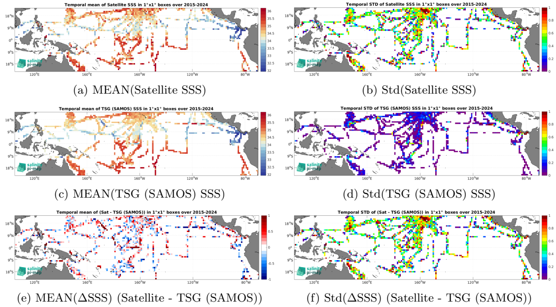
Figure 7: Temporal mean (left) and Std (right) of SSS from SMAP SSS L2 v6 - 40 km (RSS) (top), TSG (SAMOS) (middle), and of \Delta SSS (Satellite - TSG (SAMOS)). Only match-up pairs are used to generate these maps.
