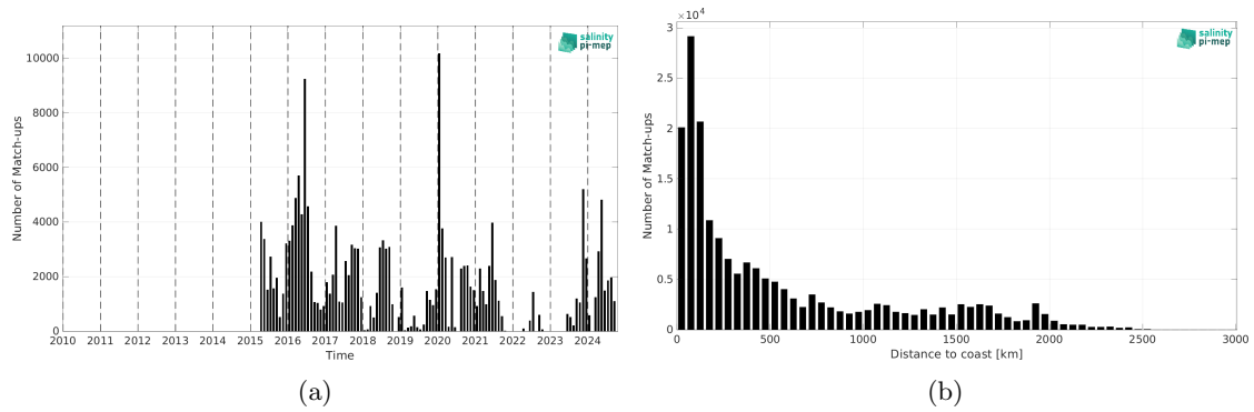
Figure 2: Number of match-ups between TSG (SAMOS) and SMAP SSS L2 v6 - 40 km (RSS) SSS as a function of time (a) and as function of the distance to coast (b) over the Tropical Pacific Ocean Pi-MEP region and for the full satellite product period.
