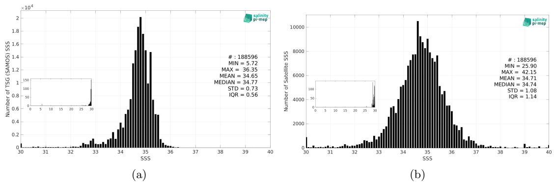
Figure 3: Histograms of SSS from TSG (SAMOS) (a) and SMAP SSS L2 v6 - 40 km (RSS) (b) considering all match-up pairs per bins of 0.1 over the Tropical Pacific Ocean Pi-MEP region and for the full satellite product period.
