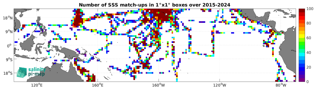
Figure 5: Number of SSS match-ups between TSG (SAMOS) SSS and the SMAP SSS L2 v6 - 40 km (RSS) SSS product for the Tropical Pacific Ocean Pi-MEP region over 1^\circ \times 1^\circ boxes and for the full satellite product period.
