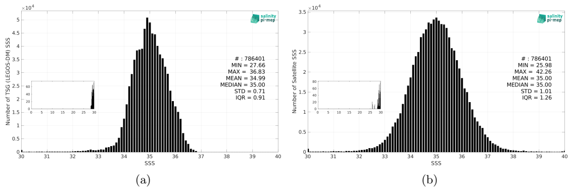
Figure 3: Histograms of SSS from TSG (LEGOS-DM) (a) and SMAP SSS L2 v6 - 40 km (RSS) (b) considering all match-up pairs per bins of 0.1 over the Tropical Pacific Ocean Pi-MEP region and for the full satellite product period.
