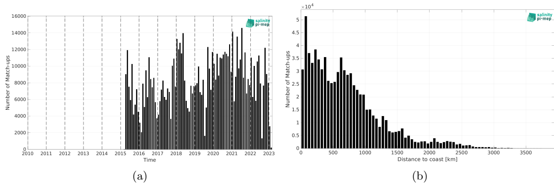
Figure 2: Number of match-ups between TSG (LEGOS-DM) and SMAP SSS L2 v6 - 40 km (RSS) SSS as a function of time (a) and as function of the distance to coast (b) over the Tropical Pacific Ocean Pi-MEP region and for the full satellite product period.
