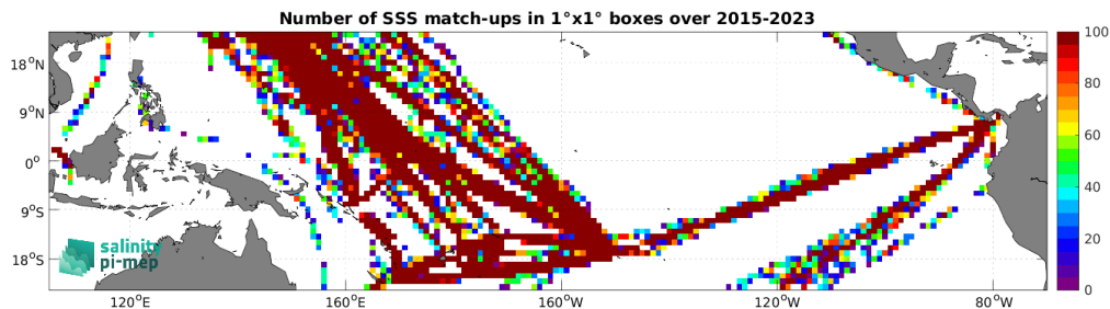
Figure 5: Number of SSS match-ups between TSG (LEGOS-DM) SSS and the SMAP SSS L2 v6 - 40 km (RSS) SSS product for the Tropical Pacific Ocean Pi-MEP region over 1^\circ \times 1^\circ boxes and for the full satellite product period.
