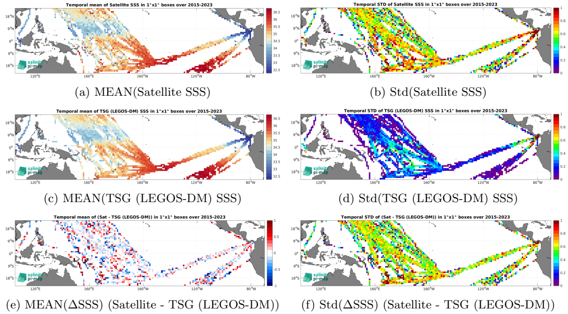
Figure 7: Temporal mean (left) and Std (right) of SSS from SMAP SSS L2 v6 - 40 km (RSS) (top), TSG (LEGOS-DM) (middle), and of \Delta SSS (Satellite - TSG (LEGOS-DM)). Only match-up pairs are used to generate these maps.
