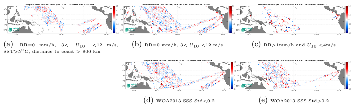
Figure 14: Temporal mean gridded over spatial boxes of size 1^\circ \times 1^\circ of \Delta\text{SSS} (SMAP SSS L2 v6 - 40 km (RSS) - TSG (LEGOS-DM)) for 5 different subdatasets corresponding to: RR=0 mm/h, 3 < U_{10} < 12 m/s, SST > 5°C, distance to coast > 800 km (a), RR=0 mm/h, 3 < U_{10} < 12 m/s (b), RR > 1mm/h and U_{10} < 4 m/s (c), WOA2013 SSS Std < 0.2 (d), WOA2013 SSS Std > 0.2 (e).
