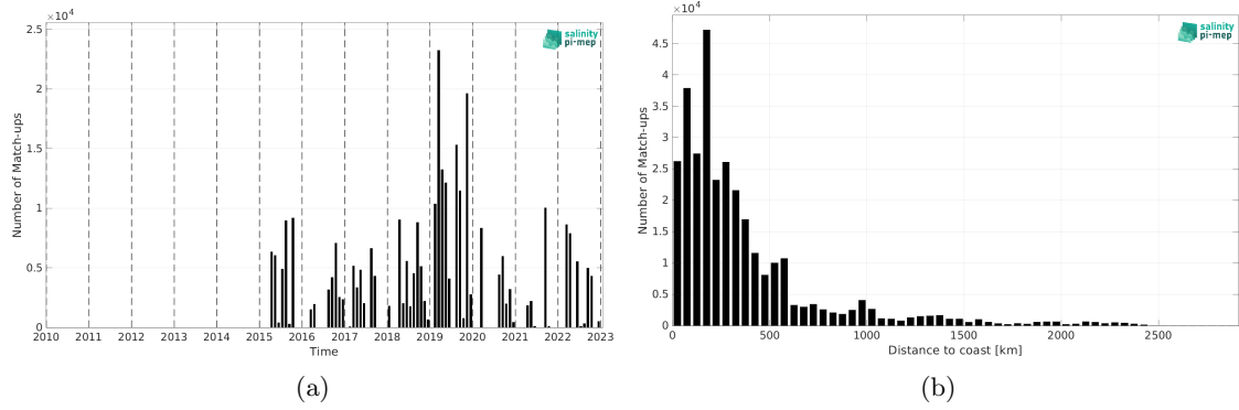
Figure 2: Number of match-ups between TSG (GOSUD-Research-vessel) and SMAP SSS L2 v6 - 40 km (RSS) SSS as a function of time (a) and as function of the distance to coast (b) over the Tropical Pacific Ocean Pi-MEP region and for the full satellite product period.
