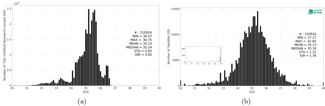
Figure 3: Histograms of SSS from TSG (GOSUD-Research-vessel) (a) and SMAP SSS L2 v6 - 40 km (RSS) (b) considering all match-up pairs per bins of 0.1 over the Tropical Pacific Ocean Pi-MEP region and for the full satellite product period.
