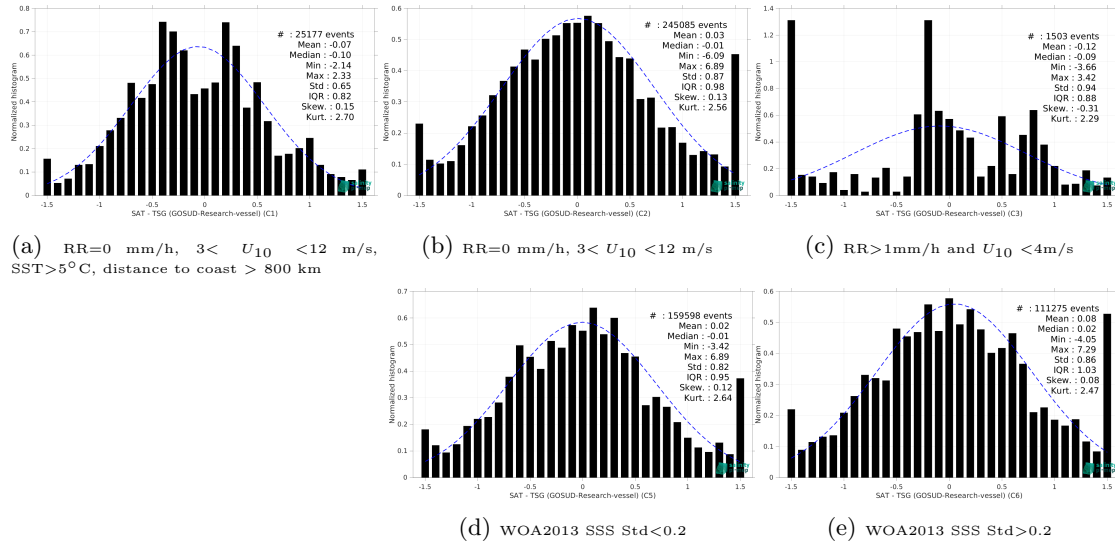
Figure 15: Normalized histogram of \Delta SSS (SMAP SSS L2 v6 - 40 km (RSS) - TSG (GOSUD-Research-vessel)) for 5 different subdatasets corresponding to: RR=0 mm/h, 3 < U_{10} < 12 m/s, SST >5^{\circ} C, distance to coast > 800 km (a), RR=0 mm/h, 3 < U_{10} < 12 m/s (b), RR >1 mm/h and U_{10} < 4 m/s (c), WOA2013 SSS Std <0.2 (d), WOA2013 SSS Std >0.2 (e).
