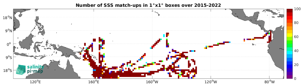
Figure 5: Number of SSS match-ups between TSG (GOSUD-Research-vessel) SSS and the SMAP SSS L2 v6 - 40 km (RSS) SSS product for the Tropical Pacific Ocean Pi-MEP region over 1^\circ \times 1^\circ boxes and for the full satellite product period.
