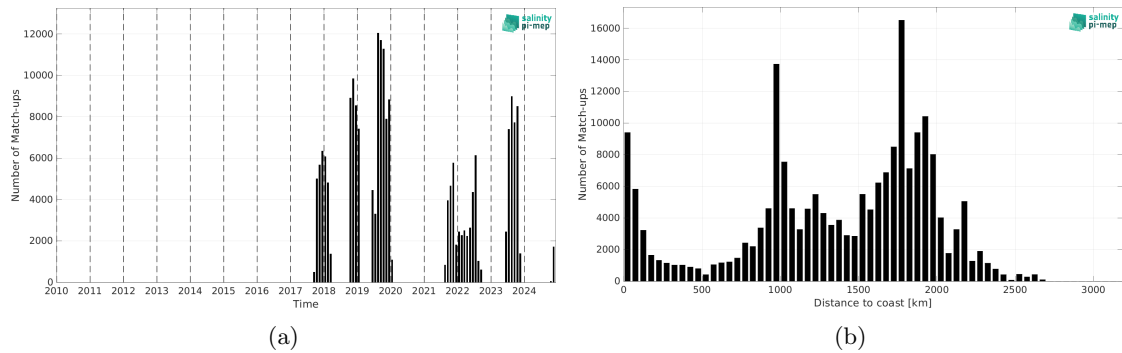
Figure 2: Number of match-ups between Sairdrone and SMAP SSS L2 v6 - 40 km (RSS) SSS as a function of time (a) and as function of the distance to coast (b) over the Tropical Pacific Ocean Pi-MEP region and for the full satellite product period.
