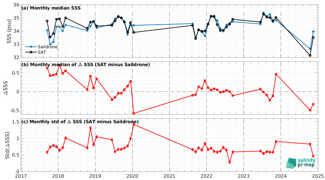
Figure 8: Time series of the monthly median SSS (top), median of \Delta SSS (Satellite - Sairdrone) and Std of \Delta SSS (Satellite - Sairdrone) over the Tropical Pacific Ocean Pi-MEP region considering all match-ups collected by the Pi-MEP.
