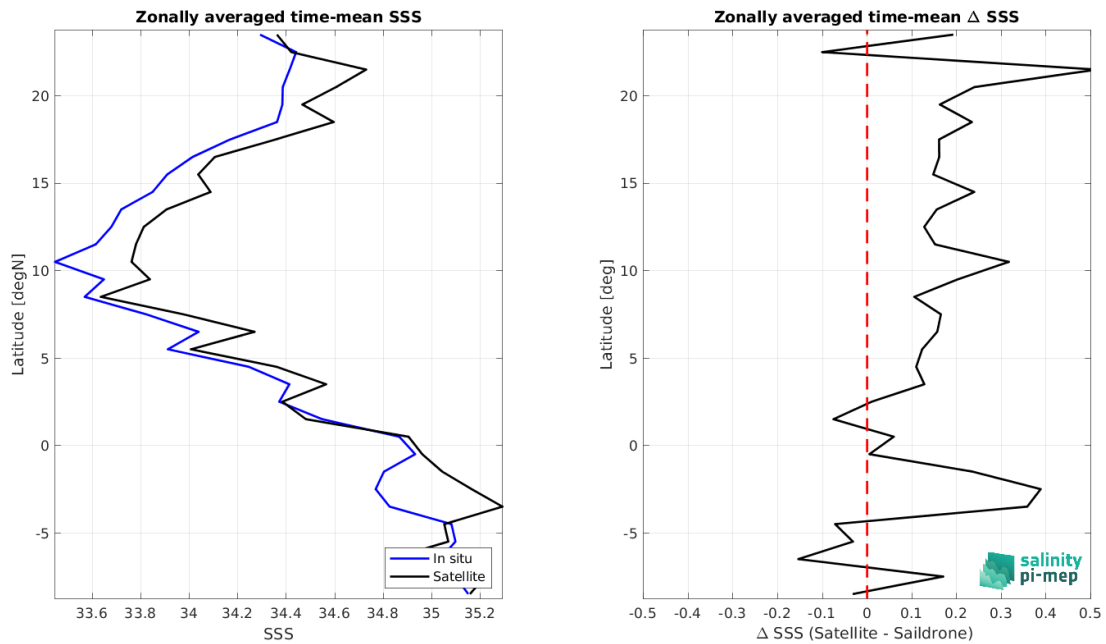
Figure 9: Left panel: Zonal mean SSS from SMAP SSS L2 v6 - 40 km (RSS) satellite product (black) and from Saildrone (blue). Right panel: Zonal mean of \Delta SSS (Satellite - Saildrone) for all the collected Pi-MEP match-up pairs estimated over the full satellite product period.
