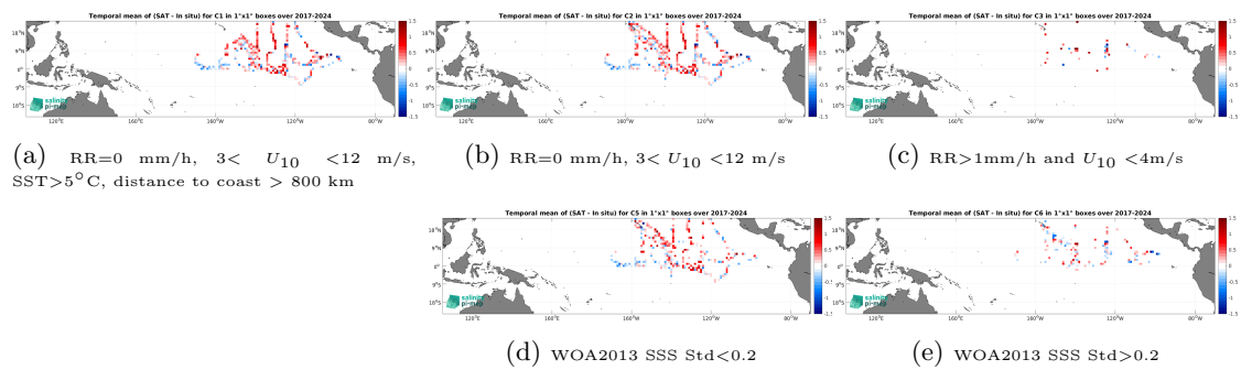
Figure 14: Temporal mean gridded over spatial boxes of size 1^\circ \times 1^\circ of \Delta SSS (SMAP SSS L2 v6 - 40 km (RSS) - Sairdrone) for 5 different subdatasets corresponding to:RR=0 mm/h, 3 < U_{10} < 12 m/s, SST > 5^\circ\text{C} , distance to coast > 800 km (a), RR=0 mm/h, 3 < U_{10} < 12 m/s (b), RR > 1 mm/h and U_{10} < 4 m/s (c), WOA2013 SSS Std < 0.2 (d), WOA2013 SSS Std > 0.2 (e).
