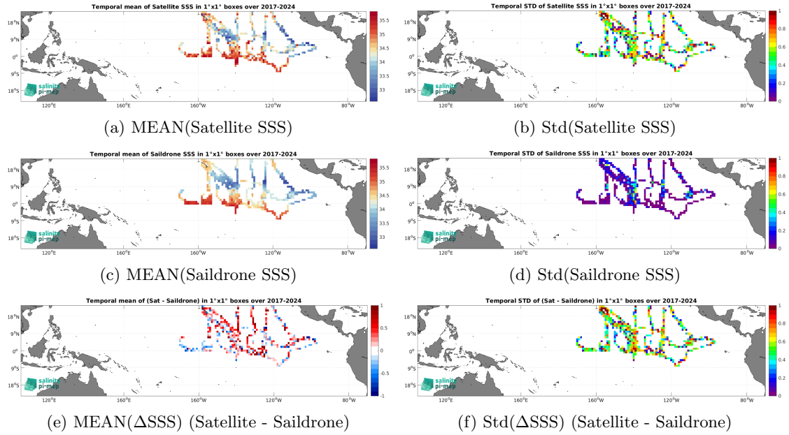
Figure 7: Temporal mean (left) and Std (right) of SSS from SMAP SSS L2 v6 - 40 km (RSS) (top), Saildrone (middle), and of \Delta SSS (Satellite - Saildrone). Only match-up pairs are used to generate these maps.
