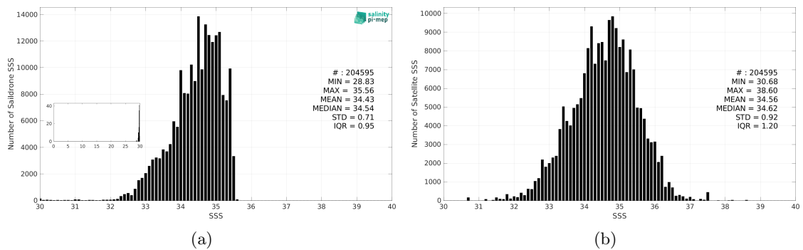
Figure 3: Histograms of SSS from Sairdrone (a) and SMAP SSS L2 v6 - 40 km (RSS) (b) considering all match-up pairs per bins of 0.1 over the Tropical Pacific Ocean Pi-MEP region and for the full satellite product period.
