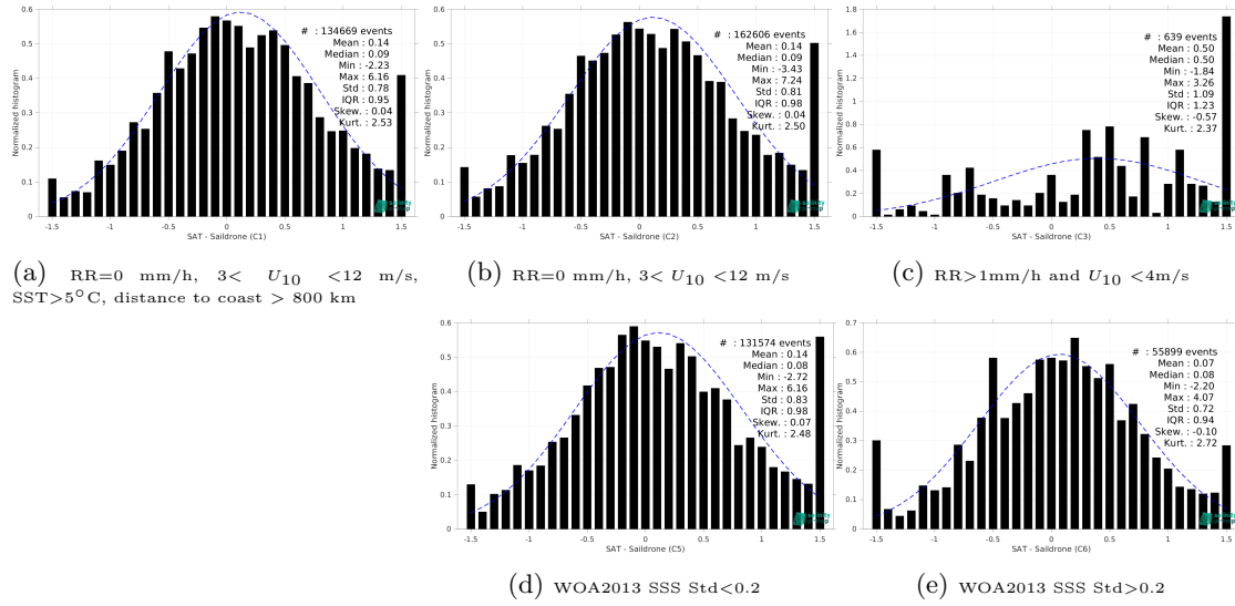
Figure 15: Normalized histogram of \Delta SSS (SMAP SSS L2 v6 - 40 km (RSS) - Saildrone) for 5 different subdatasets corresponding to: RR=0 mm/h, 3 < U_{10} < 12 m/s, SST>5°C, distance to coast > 800 km (a), RR=0 mm/h, 3 < U_{10} < 12 m/s (b), RR>1mm/h and U_{10} < 4 m/s (c), WOA2013 SSS Std<0.2 (d), WOA2013 SSS Std>0.2 (e).
