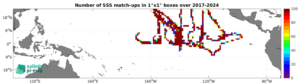
Figure 5: Number of SSS match-ups between Saildrone SSS and the SMAP SSS L2 v6 - 40 km (RSS) SSS product for the Tropical Pacific Ocean Pi-MEP region over 1^\circ \times 1^\circ boxes and for the full satellite product period.
