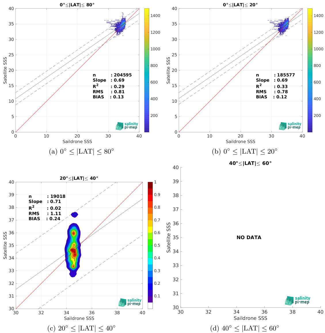
Figure 10: Contour maps of the concentration of SMAP SSS L2 v6 - 40 km (RSS) SSS (y-axis) versus Saildrone SSS (x-axis) at match-up pairs for different latitude bands. For each plot, the red line shows x=y . The black thin and dashed lines indicate a linear fit through the data cloud and the \pm 95\% confidence levels, respectively. The number match-up pairs n , the slope and R^2 coefficient of the linear fit, the root mean square (RMS) and the mean bias between satellite and in situ data are indicated for each latitude band in each plots.
