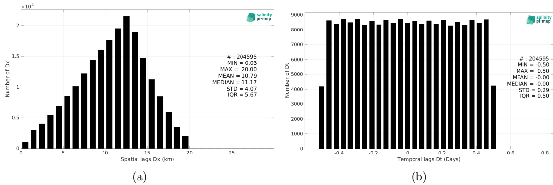
Figure 6: Histograms of the spatial (a) and temporal (b) lags between the location/time of the Saildrone measurement and the date of the corresponding SMAP SSS L2 v6 - 40 km (RSS) SSS pixel.
