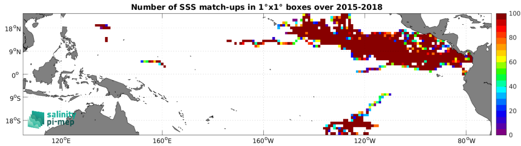
Figure 4: Number of SSS match-ups between Surface drifters SSS and the SMAP SSS L2 v6 - 40 km (RSS) SSS product for the Tropical Pacific Ocean Pi-MEP region over 1^\circ \times 1^\circ boxes and for the full satellite product period.
