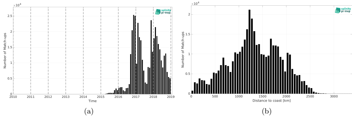
Figure 2: Number of match-ups between Surface drifters and SMAP SSS L2 v6 - 40 km (RSS) SSS as a function of time (a) and as function of the distance to coast (b) over the Tropical Pacific Ocean Pi-MEP region and for the full satellite product period.
