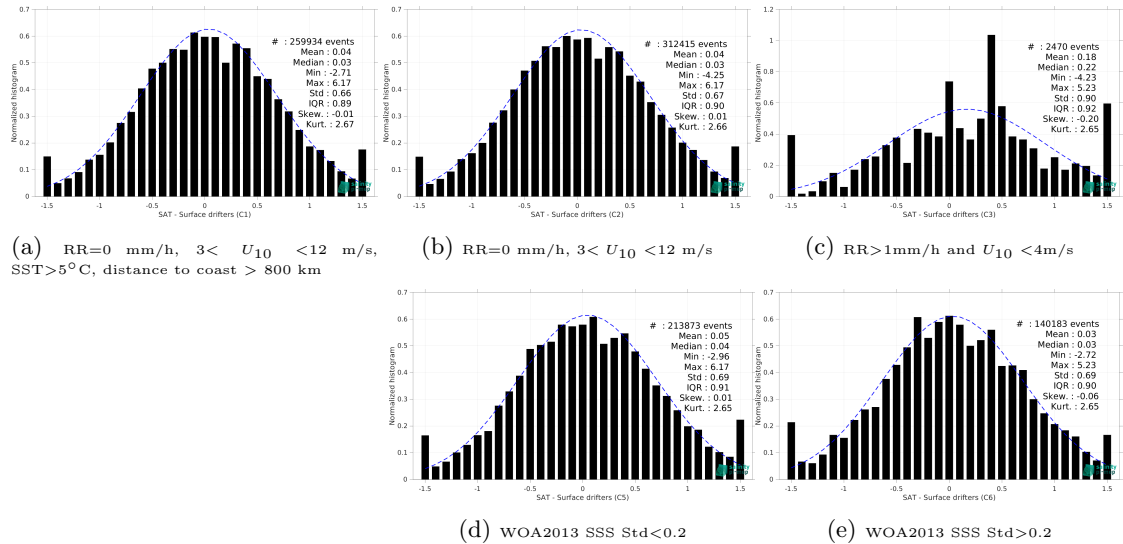
Figure 14: Normalized histogram of \Delta SSS (SMAP SSS L2 v6 - 40 km (RSS) - Surface drifters) for 5 different subdatasets corresponding to: RR=0 mm/h, 3 < U_{10} < 12 m/s, SST >5^\circ\text{C} , distance to coast > 800 km (a), RR=0 mm/h, 3 < U_{10} < 12 m/s (b), RR >1 mm/h and U_{10} < 4 m/s (c), WOA2013 SSS Std <0.2 (d), WOA2013 SSS Std >0.2 (e).
