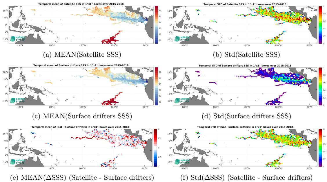
Figure 6: Temporal mean (left) and Std (right) of SSS from SMAP SSS L2 v6 - 40 km (RSS) (top), Surface drifters (middle), and of \Delta SSS (Satellite - Surface drifters). Only match-up pairs are used to generate these maps.
