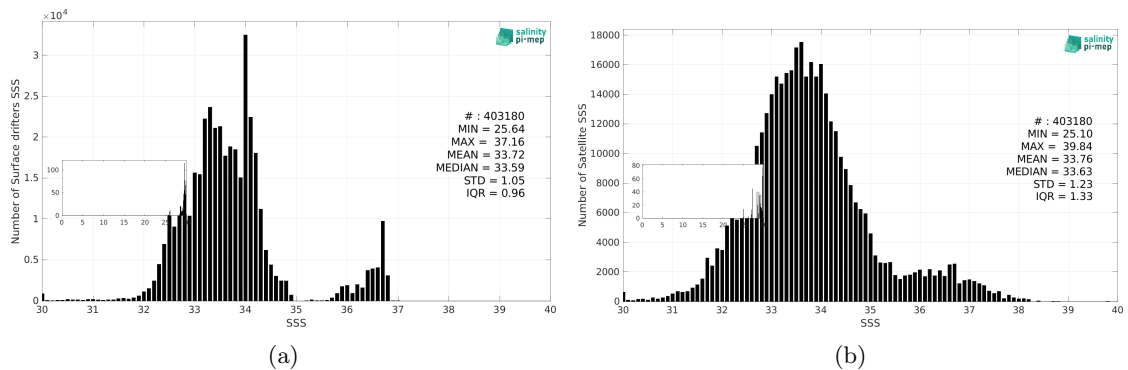
Figure 3: Histograms of SSS from Surface drifters (a) and SMAP SSS L2 v6 - 40 km (RSS) (b) considering all match-up pairs per bins of 0.1 over the Tropical Pacific Ocean Pi-MEP region and for the full satellite product period.
