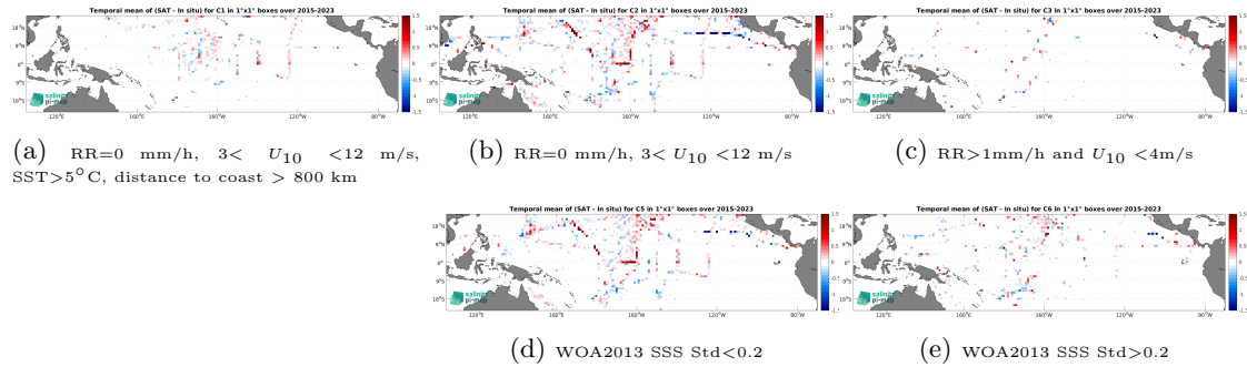
Figure 12: Temporal mean gridded over spatial boxes of size 1^\circ \times 1^\circ of \Delta SSS (SMAP SSS L2 v5 (RSS) - TSG (SAMOS)) for 5 different subdatasets corresponding to:RR=0 mm/h, 3 < U_{10} < 12 m/s, SST>5°C, distance to coast > 800 km (a), RR=0 mm/h, 3 < U_{10} < 12 m/s (b), RR>1mm/h and U_{10} < 4 m/s (c), WOA2013 SSS Std<0.2 (d), WOA2013 SSS Std>0.2 (e).
