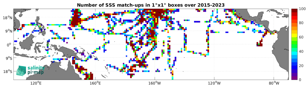
Figure 4: Number of SSS match-ups between TSG (SAMOS) SSS and the SMAP SSS L2 v5 (RSS) SSS product for the Tropical Pacific Ocean Pi-MEP region over 1^\circ \times 1^\circ boxes and for the full satellite product period.
