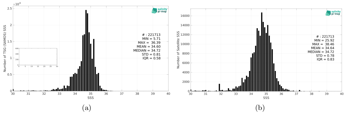
Figure 2: Histograms of SSS from TSG (SAMOS) (a) and SMAP SSS L2 v5 (RSS) (b) considering all match-up pairs per bins of 0.1 over the Tropical Pacific Ocean Pi-MEP region and for the full satellite product period.
