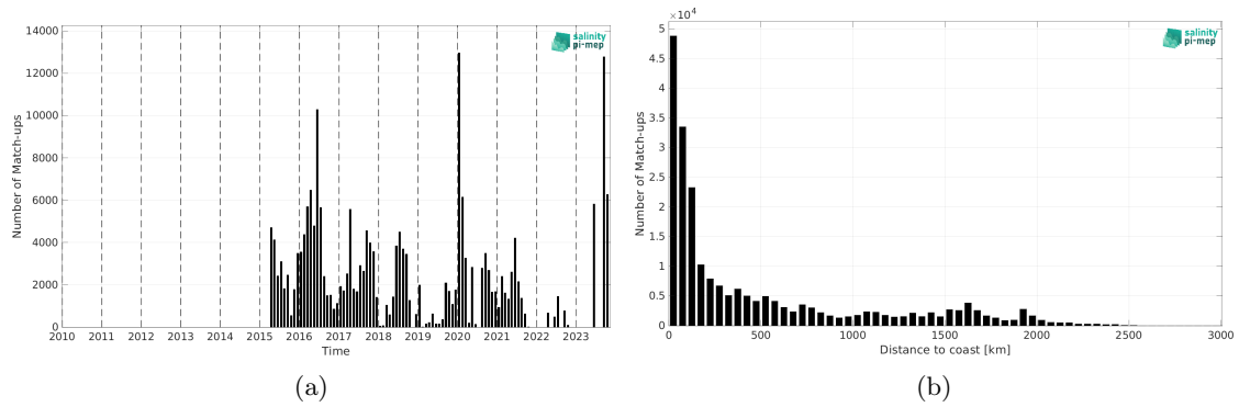
Figure 1: Number of match-ups between TSG (SAMOS) and SMAP SSS L2 v5 (RSS) SSS as a function of time (a) and as function of the distance to coast (b) over the Tropical Pacific Ocean Pi-MEP region and for the full satellite product period.
