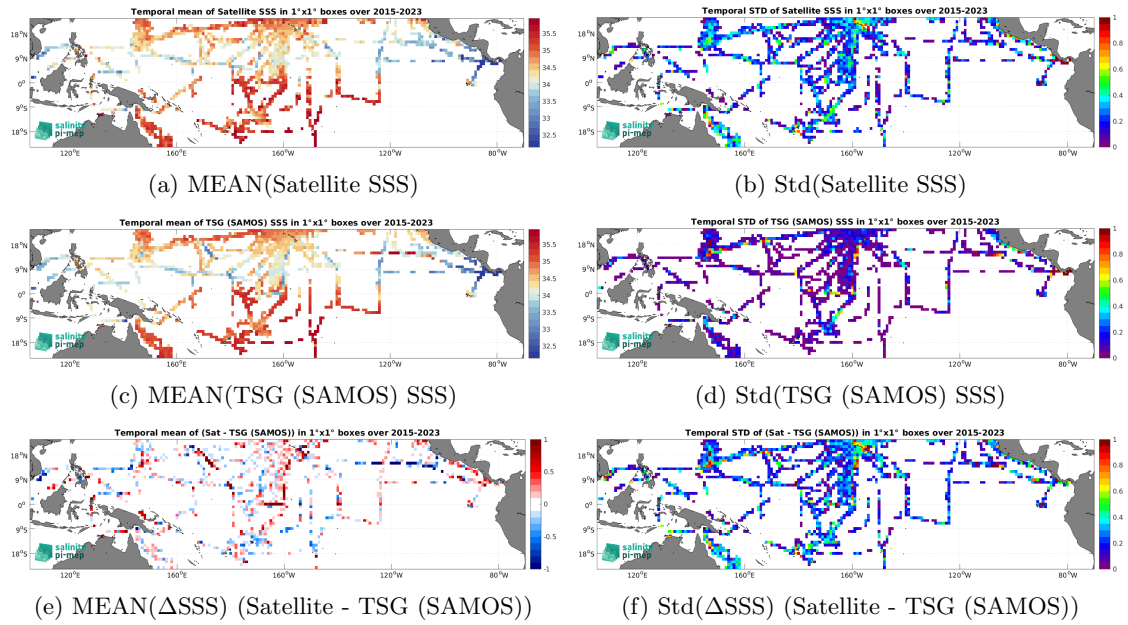
Figure 6: Temporal mean (left) and Std (right) of SSS from SMAP SSS L2 v5 (RSS) (top), TSG (SAMOS) (middle), and of \Delta SSS (Satellite - TSG (SAMOS)). Only match-up pairs are used to generate these maps.
