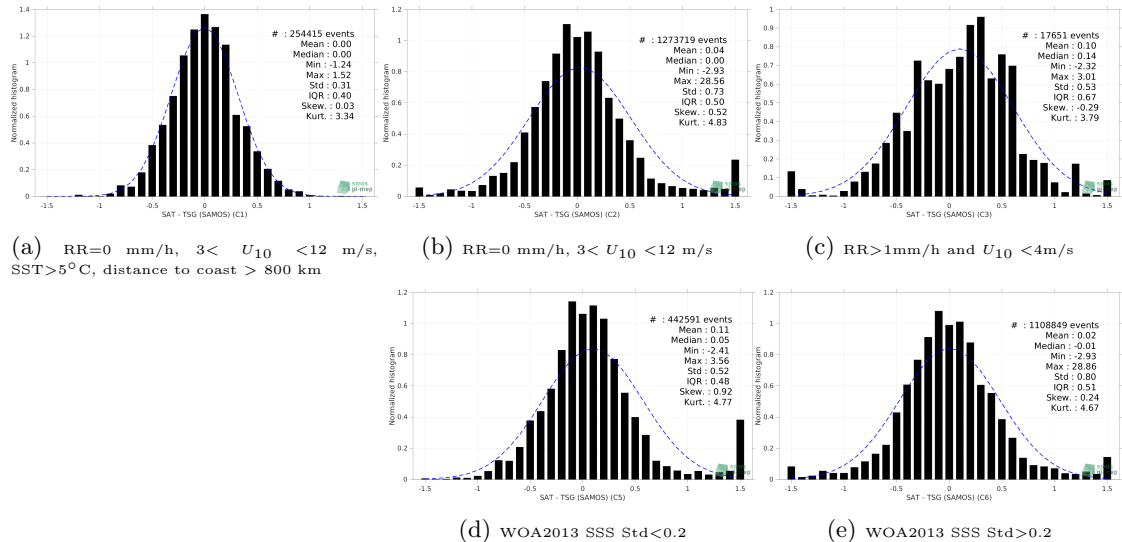
Figure 13: Normalized histogram of \Delta SSS (SMAP SSS L2 v5 (RSS) - TSG (SAMOS)) for 5 different subdatasets corresponding to: RR=0 mm/h, 3 < U_{10} < 12 m/s, SST >5^\circ C, distance to coast > 800 km (a), RR=0 mm/h, 3 < U_{10} < 12 m/s (b), RR >1 mm/h and U_{10} < 4 m/s (c), WOA2013 SSS Std <0.2 (d), WOA2013 SSS Std >0.2 (e).
