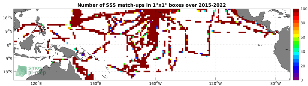
Figure 4: Number of SSS match-ups between TSG (SAMOS) SSS and the SMAP SSS L2 v5 (RSS) SSS product for the Tropical Pacific Ocean Pi-MEP region over 1^\circ \times 1^\circ boxes and for the full satellite product period.
