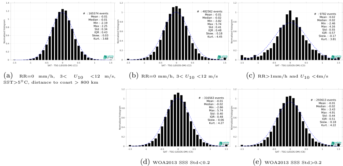
Figure 13: Normalized histogram of \Delta\text{SSS} (SMAP SSS L2 v5 (RSS) - TSG (LEGOS-DM)) for 5 different subdatasets corresponding to: RR=0 mm/h, 3 < U_{10} < 12 m/s, SST >5^\circ\text{C} , distance to coast > 800 km (a), RR=0 mm/h, 3 < U_{10} < 12 m/s (b), RR >1 mm/h and U_{10} < 4 m/s (c), WOA2013 SSS Std <0.2 (d), WOA2013 SSS Std >0.2 (e).
