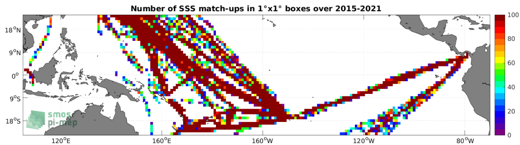
Figure 4: Number of SSS match-ups between TSG (LEGOS-DM) SSS and the SMAP SSS L2 v5 (RSS) SSS product for the Tropical Pacific Ocean Pi-MEP region over 1^\circ \times 1^\circ boxes and for the full satellite product period.
