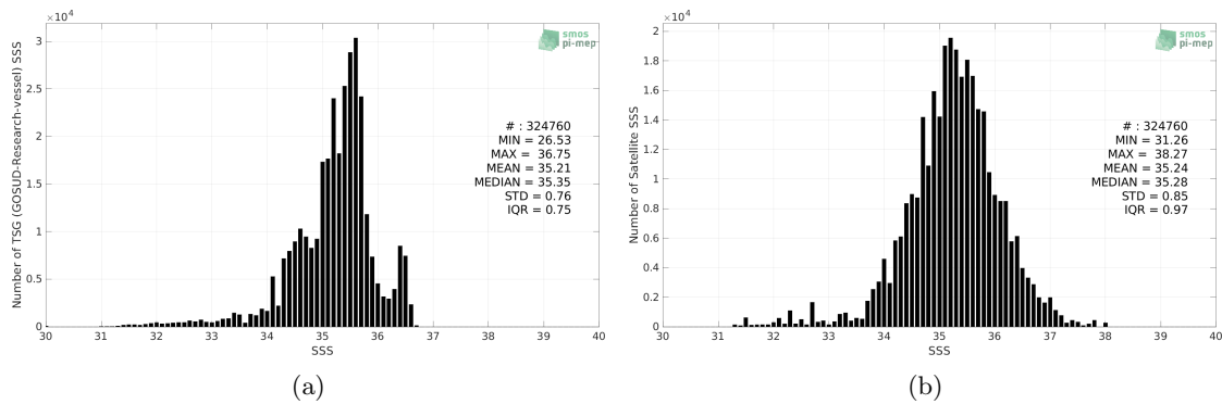
Figure 2: Histograms of SSS from TSG (GOSUD-Research-vessel) (a) and SMAP SSS L2 v5 (RSS) (b) considering all match-up pairs per bins of 0.1 over the Tropical Pacific Ocean Pi-MEP region and for the full satellite product period.
