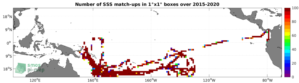
Figure 4: Number of SSS match-ups between TSG (GOSUD-Research-vessel) SSS and the SMAP SSS L2 v5 (RSS) SSS product for the Tropical Pacific Ocean Pi-MEP region over 1^\circ \times 1^\circ boxes and for the full satellite product period.
