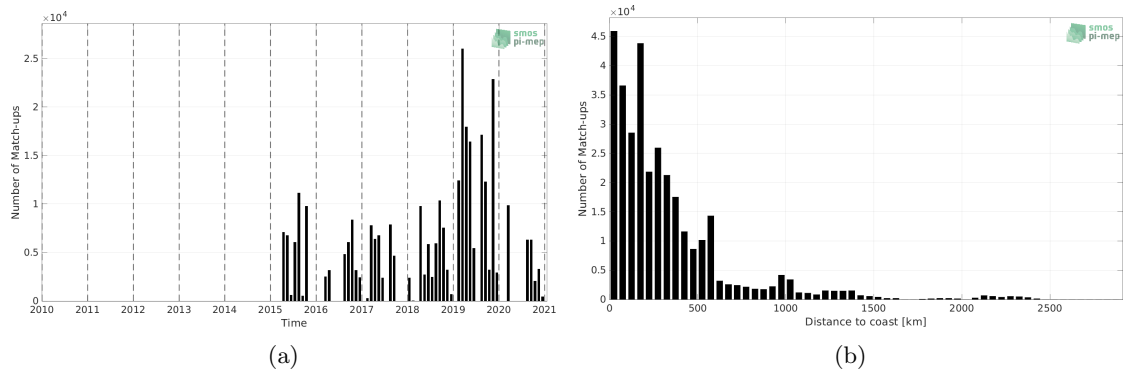
Figure 1: Number of match-ups between TSG (GOSUD-Research-vessel) and SMAP SSS L2 v5 (RSS) SSS as a function of time (a) and as function of the distance to coast (b) over the Tropical Pacific Ocean Pi-MEP region and for the full satellite product period.
