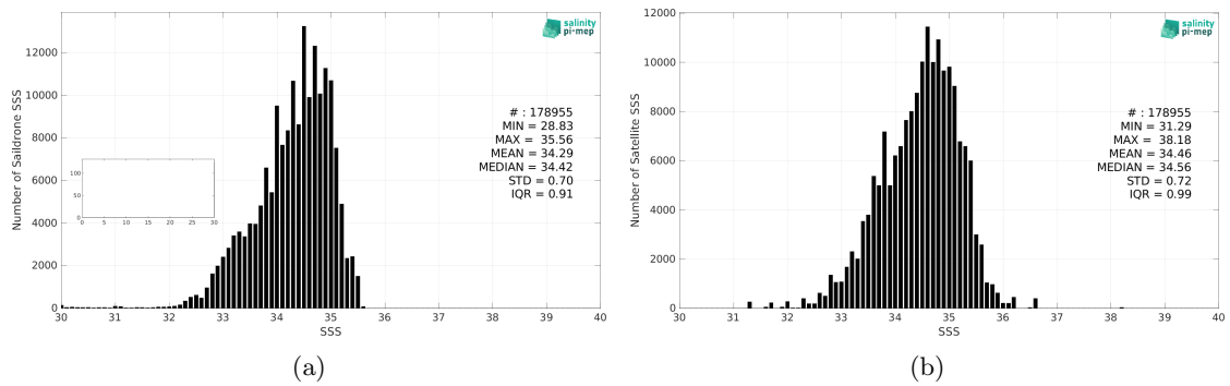
Figure 2: Histograms of SSS from Saildrone (a) and SMAP SSS L2 v5 (RSS) (b) considering all match-up pairs per bins of 0.1 over the Tropical Pacific Ocean Pi-MEP region and for the full satellite product period.
