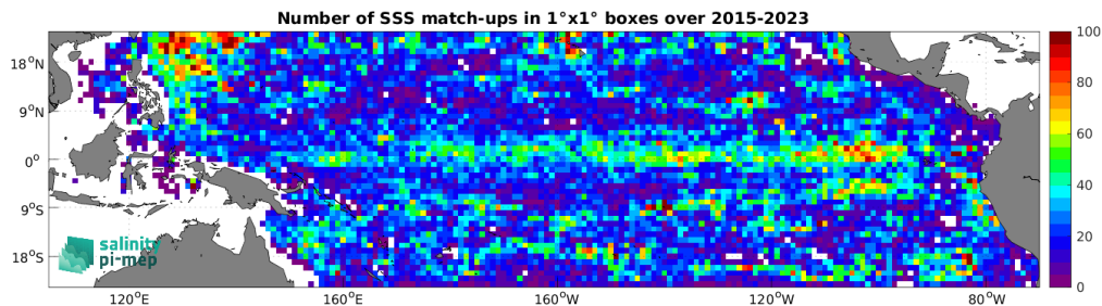
Figure 4: Number of SSS match-ups between Argo SSS and the SMAP SSS L2 v5 (RSS) SSS product for the Tropical Pacific Ocean Pi-MEP region over 1^\circ \times 1^\circ boxes and for the full satellite product period.
