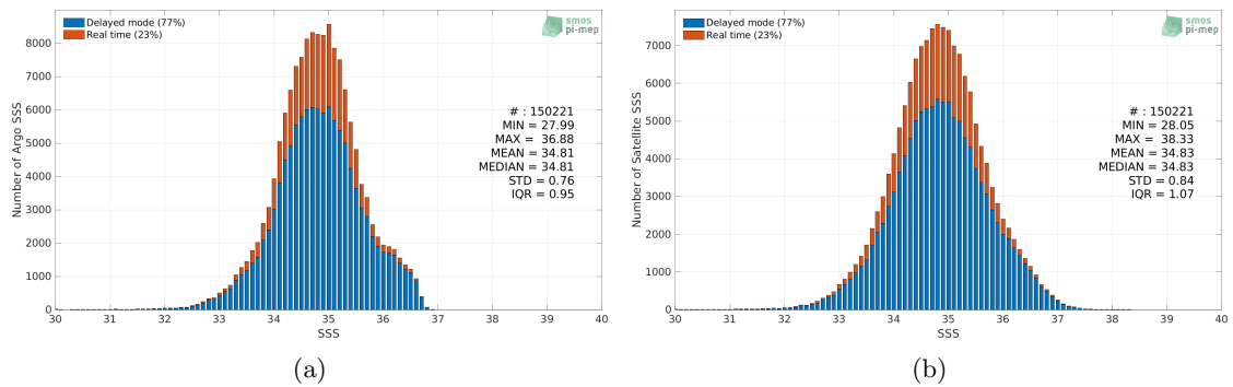
Figure 2: Histograms of SSS from Argo (a) and SMAP SSS L2 v5 (RSS) (b) considering all match-up pairs per bins of 0.1 over the Tropical Pacific Ocean Pi-MEP region and for the full satellite product period.
