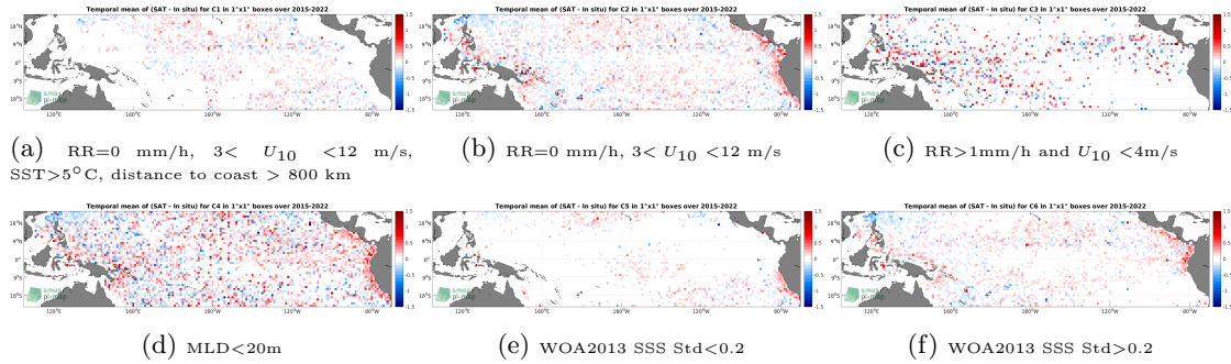
Figure 12: Temporal mean gridded over spatial boxes of size 1^\circ \times 1^\circ of \Delta SSS (SMAP SSS L2 v5 (RSS) - Argo) for 6 different subdatasets corresponding to:RR=0 mm/h, 3 < U_{10} < 12 m/s, SST >5^\circ C, distance to coast > 800 km (a), RR=0 mm/h, 3 < U_{10} < 12 m/s (b), RR >1 mm/h and U_{10} < 4 m/s (c),MLD <20 m (d),WOA2013 SSS Std <0.2 (e),WOA2013 SSS Std >0.2 (f).
