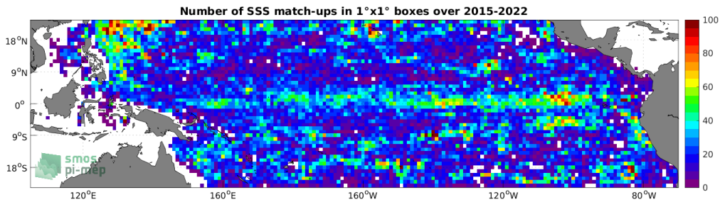
Figure 4: Number of SSS match-ups between Argo SSS and the SMAP SSS L2 v5 (RSS) SSS product for the Tropical Pacific Ocean Pi-MEP region over 1^\circ \times 1^\circ boxes and for the full satellite product period.
