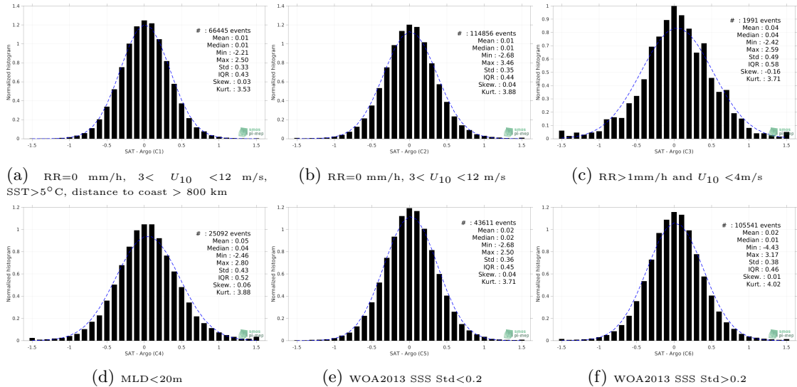
Figure 13: Normalized histogram of \Delta SSS (SMAP SSS L2 v5 (RSS) - Argo) for 6 different subdatasets corresponding to: RR=0 mm/h, 3 < U_{10} < 12 m/s, SST >5^\circ C, distance to coast > 800 km (a), RR=0 mm/h, 3 < U_{10} < 12 m/s (b), RR >1 mm/h and U_{10} < 4 m/s (c), MLD <20 m (d), WOA2013 SSS Std <0.2 (e), WOA2013 SSS Std >0.2 (f).
