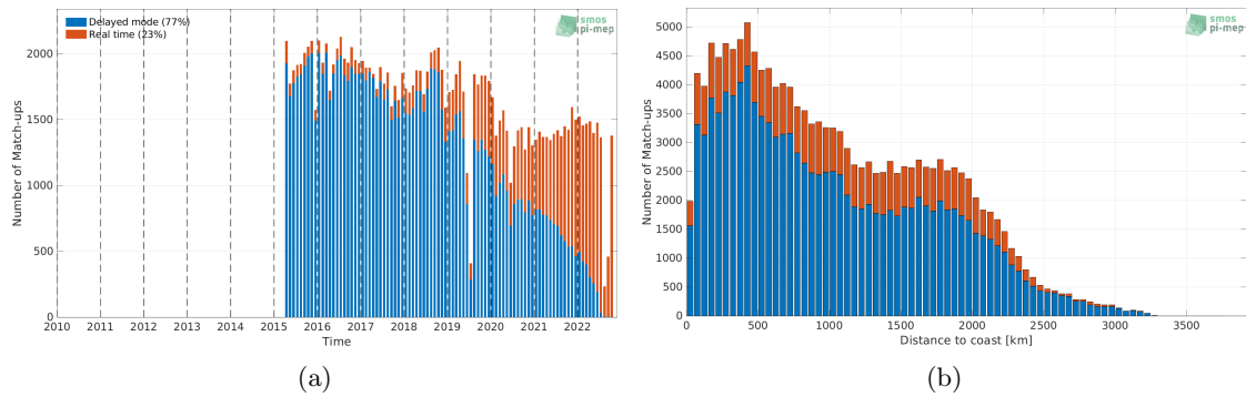
Figure 1: Number of match-ups between Argo and SMAP SSS L2 v5 (RSS) SSS as a function of time (a) and as function of the distance to coast (b) over the Tropical Pacific Ocean Pi-MEP region and for the full satellite product period.
