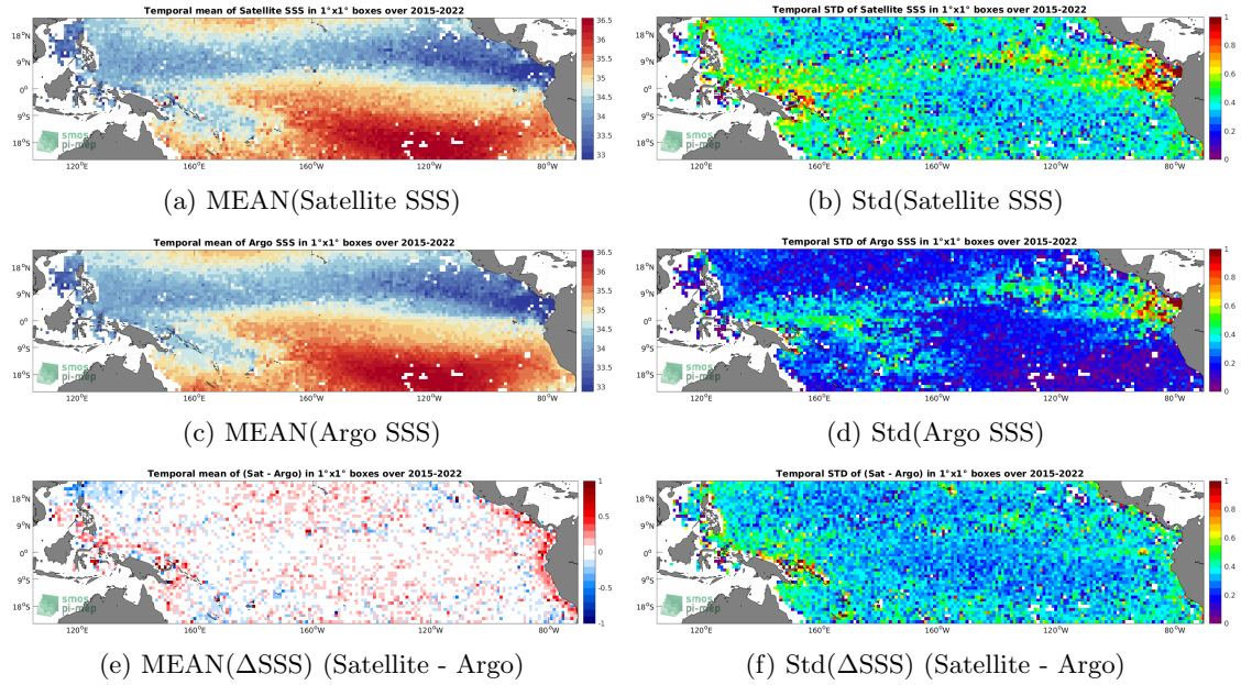
Figure 6: Temporal mean (left) and Std (right) of SSS from SMAP SSS L2 v5 (RSS) (top), Argo (middle), and of \Delta SSS (Satellite - Argo). Only match-up pairs are used to generate these maps.
