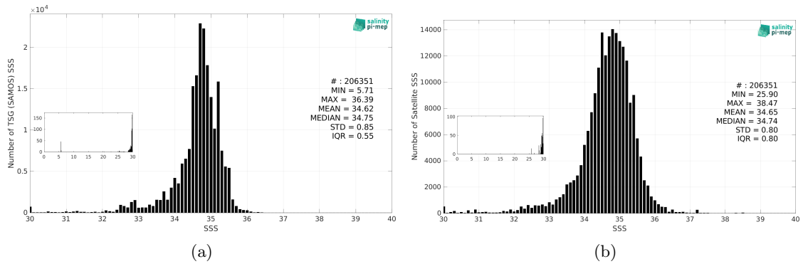
Figure 3: Histograms of SSS from TSG (SAMOS) (a) and SMAP SSS L2 v5.3 (RSS) (b) considering all match-up pairs per bins of 0.1 over the Tropical Pacific Ocean Pi-MEP region and for the full satellite product period.
