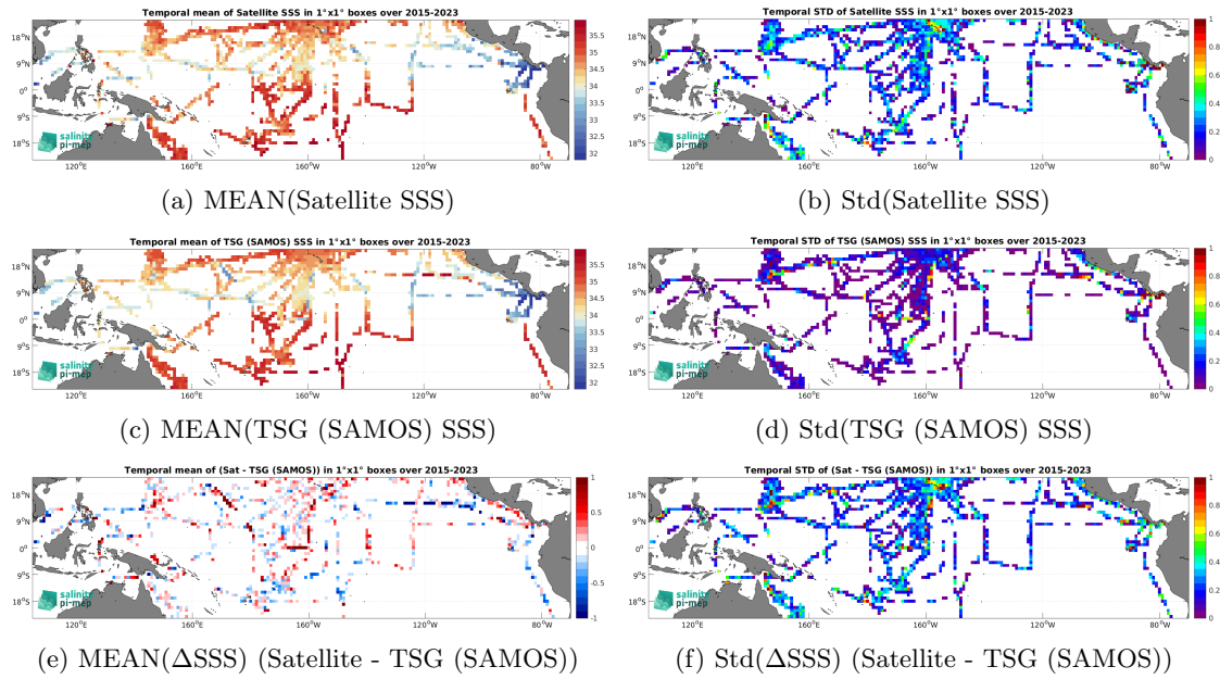
Figure 7: Temporal mean (left) and Std (right) of SSS from SMAP SSS L2 v5.3 (RSS) (top), TSG (SAMOS) (middle), and of \Delta SSS (Satellite - TSG (SAMOS)). Only match-up pairs are used to generate these maps.
