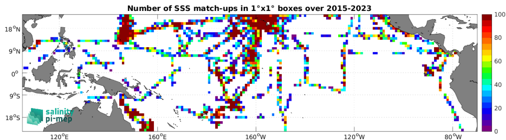
Figure 5: Number of SSS match-ups between TSG (SAMOS) SSS and the SMAP SSS L2 v5.3 (RSS) SSS product for the Tropical Pacific Ocean Pi-MEP region over 1^\circ \times 1^\circ boxes and for the full satellite product period.
