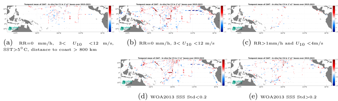
Figure 14: Temporal mean gridded over spatial boxes of size 1^\circ \times 1^\circ of \Delta SSS (SMAP SSS L2 v5.3 (RSS) - TSG (SAMOS)) for 5 different subdatasets corresponding to:RR=0 mm/h, 3 < U_{10} < 12 m/s, SST > 5^\circ\text{C} , distance to coast > 800 km (a), RR=0 mm/h, 3 < U_{10} < 12 m/s (b), RR > 1 mm/h and U_{10} < 4 m/s (c), WOA2013 SSS Std < 0.2 (d), WOA2013 SSS Std > 0.2 (e).
