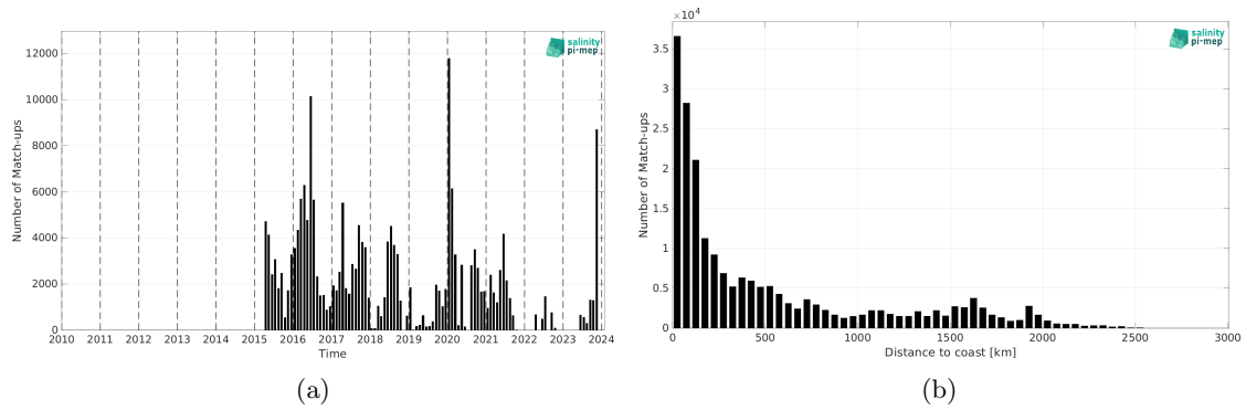
Figure 2: Number of match-ups between TSG (SAMOS) and SMAP SSS L2 v5.3 (RSS) SSS as a function of time (a) and as function of the distance to coast (b) over the Tropical Pacific Ocean Pi-MEP region and for the full satellite product period.
