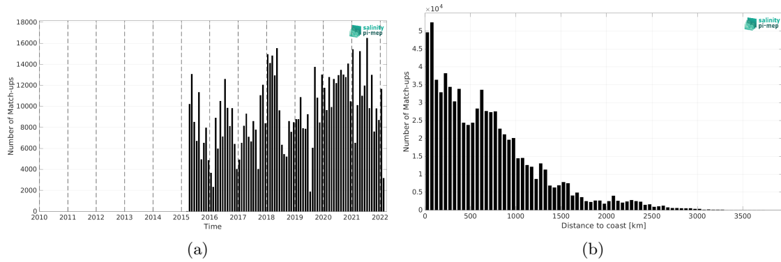
Figure 2: Number of match-ups between TSG (LEGOS-DM) and SMAP SSS L2 v5.3 (RSS) SSS as a function of time (a) and as function of the distance to coast (b) over the Tropical Pacific Ocean Pi-MEP region and for the full satellite product period.
