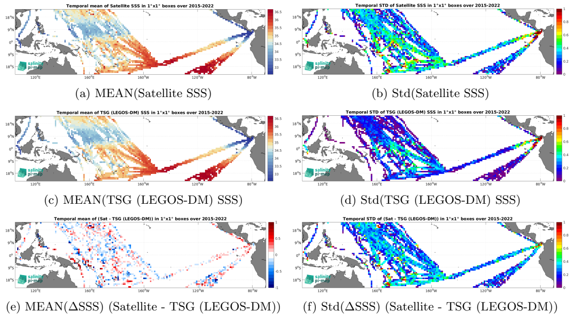
Figure 7: Temporal mean (left) and Std (right) of SSS from SMAP SSS L2 v5.3 (RSS) (top), TSG (LEGOS-DM) (middle), and of \Delta SSS (Satellite - TSG (LEGOS-DM)). Only match-up pairs are used to generate these maps.
