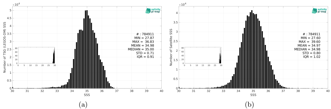
Figure 3: Histograms of SSS from TSG (LEGOS-DM) (a) and SMAP SSS L2 v5.3 (RSS) (b) considering all match-up pairs per bins of 0.1 over the Tropical Pacific Ocean Pi-MEP region and for the full satellite product period.
