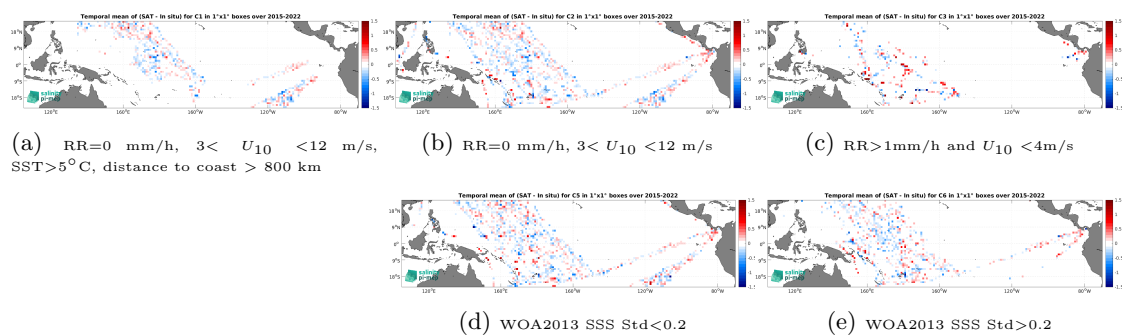
Figure 14: Temporal mean gridded over spatial boxes of size 1^\circ \times 1^\circ of \Delta SSS (SMAP SSS L2 v5.3 (RSS) - TSG (LEGOS-DM)) for 5 different subdatasets corresponding to:RR=0 mm/h, 3 < U_{10} < 12 m/s, SST > 5^\circ\text{C} , distance to coast > 800 km (a), RR=0 mm/h, 3 < U_{10} < 12 m/s (b), RR > 1 mm/h and U_{10} < 4 m/s (c), WOA2013 SSS Std < 0.2 (d), WOA2013 SSS Std > 0.2 (e).
