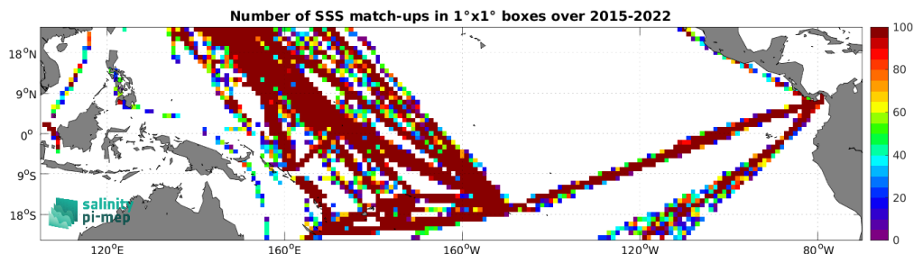
Figure 5: Number of SSS match-ups between TSG (LEGOS-DM) SSS and the SMAP SSS L2 v5.3 (RSS) SSS product for the Tropical Pacific Ocean Pi-MEP region over 1^\circ \times 1^\circ boxes and for the full satellite product period.
