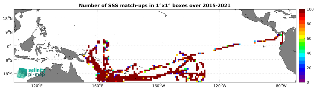
Figure 5: Number of SSS match-ups between TSG (GOSUD-Research-vessel) SSS and the SMAP SSS L2 v5.3 (RSS) SSS product for the Tropical Pacific Ocean Pi-MEP region over 1^\circ \times 1^\circ boxes and for the full satellite product period.
