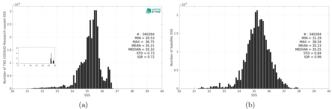
Figure 3: Histograms of SSS from TSG (GOSUD-Research-vessel) (a) and SMAP SSS L2 v5.3 (RSS) (b) considering all match-up pairs per bins of 0.1 over the Tropical Pacific Ocean Pi-MEP region and for the full satellite product period.
