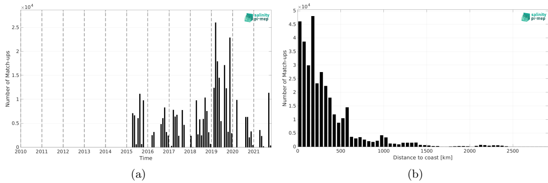
Figure 2: Number of match-ups between TSG (GOSUD-Research-vessel) and SMAP SSS L2 v5.3 (RSS) SSS as a function of time (a) and as function of the distance to coast (b) over the Tropical Pacific Ocean Pi-MEP region and for the full satellite product period.
