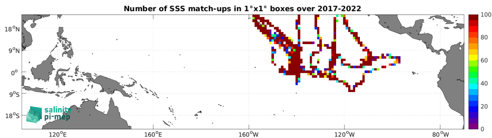
Figure 5: Number of SSS match-ups between Saildrone SSS and the SMAP SSS L2 v5.3 (RSS) SSS product for the Tropical Pacific Ocean Pi-MEP region over 1^\circ \times 1^\circ boxes and for the full satellite product period.
