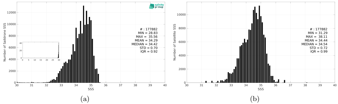
Figure 3: Histograms of SSS from Saildrone (a) and SMAP SSS L2 v5.3 (RSS) (b) considering all match-up pairs per bins of 0.1 over the Tropical Pacific Ocean Pi-MEP region and for the full satellite product period.
