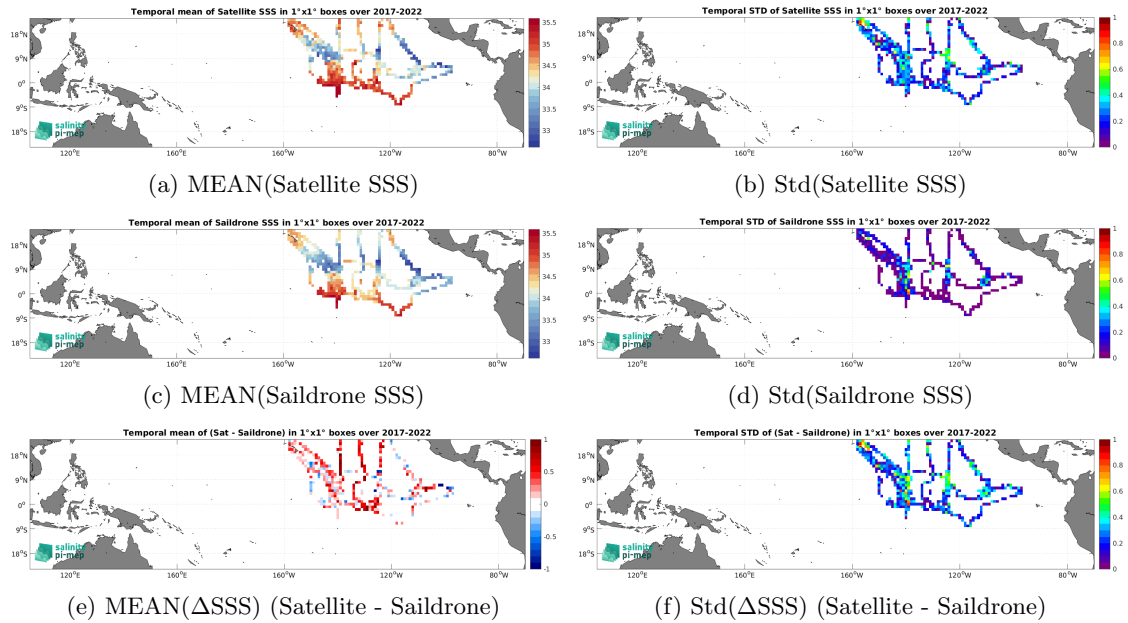
Figure 7: Temporal mean (left) and Std (right) of SSS from SMAP SSS L2 v5.3 (RSS) (top), Saildrone (middle), and of \Delta SSS (Satellite - Saildrone). Only match-up pairs are used to generate these maps.
