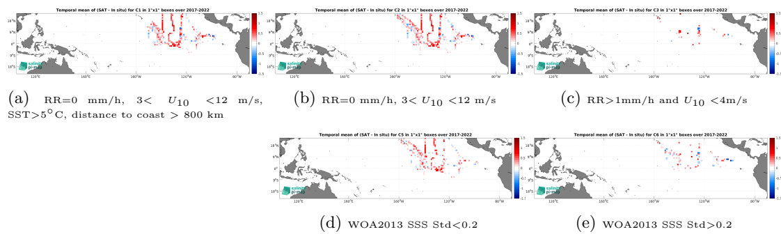
Figure 14: Temporal mean gridded over spatial boxes of size 1^\circ \times 1^\circ of \Delta SSS (SMAP SSS L2 v5.3 (RSS) - Saldrone) for 5 different subdatasets corresponding to:RR=0 mm/h, 3 < U_{10} < 12 m/s, SST > 5^\circ\text{C} , distance to coast > 800 km (a), RR=0 mm/h, 3 < U_{10} < 12 m/s (b), RR > 1 mm/h and U_{10} < 4 m/s (c), WOA2013 SSS Std < 0.2 (d), WOA2013 SSS Std > 0.2 (e).
