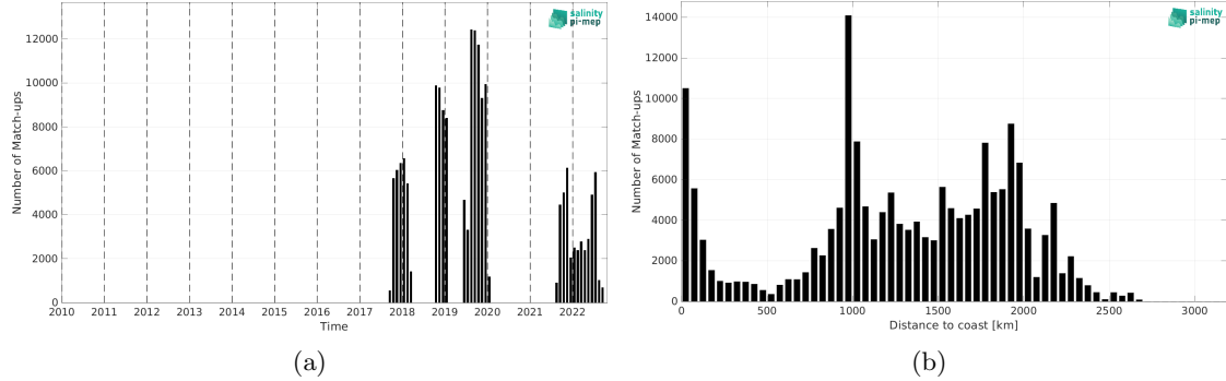
Figure 2: Number of match-ups between Saildrone and SMAP SSS L2 v5.3 (RSS) SSS as a function of time (a) and as function of the distance to coast (b) over the Tropical Pacific Ocean Pi-MEP region and for the full satellite product period.
