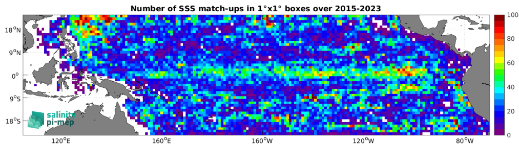
Figure 5: Number of SSS match-ups between Argo SSS and the SMAP SSS L2 v5.3 (RSS) SSS product for the Tropical Pacific Ocean Pi-MEP region over 1^\circ \times 1^\circ boxes and for the full satellite product period.
