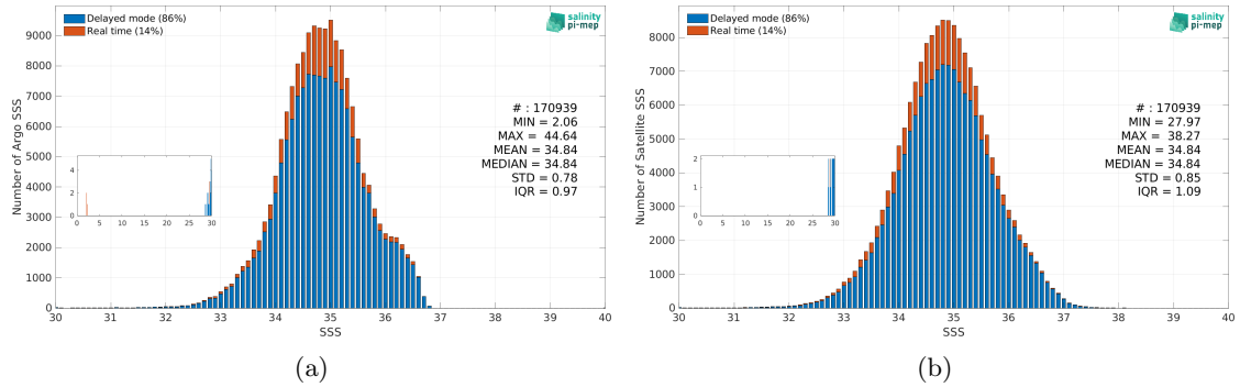
Figure 3: Histograms of SSS from Argo (a) and SMAP SSS L2 v5.3 (RSS) (b) considering all match-up pairs per bins of 0.1 over the Tropical Pacific Ocean Pi-MEP region and for the full satellite product period.
