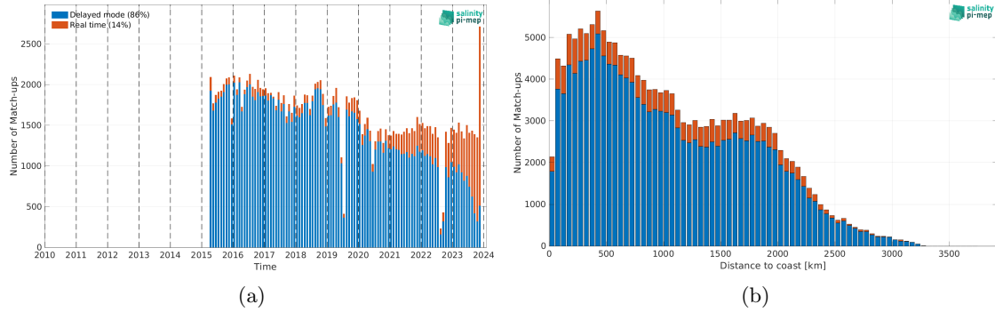
Figure 2: Number of match-ups between Argo and SMAP SSS L2 v5.3 (RSS) SSS as a function of time (a) and as function of the distance to coast (b) over the Tropical Pacific Ocean Pi-MEP region and for the full satellite product period.
