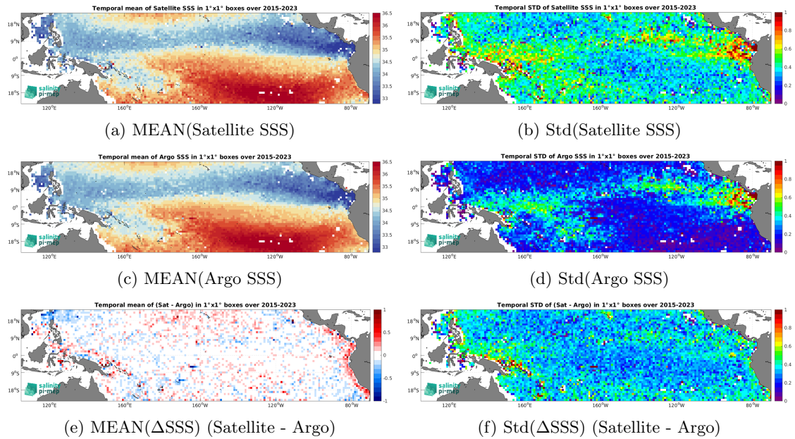
Figure 7: Temporal mean (left) and Std (right) of SSS from SMAP SSS L2 v5.3 (RSS) (top), Argo (middle), and of \Delta SSS (Satellite - Argo). Only match-up pairs are used to generate these maps.
