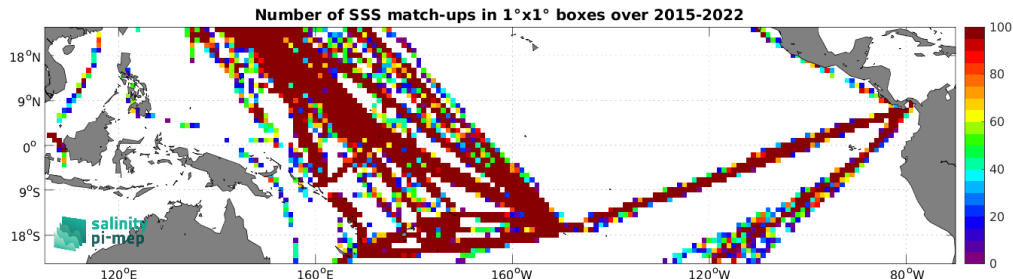
Figure 5: Number of SSS match-ups between TSG (LEGOS-DM) SSS and the SMAP SSS L2 v5.3 - 40 km (RSS) SSS product for the Tropical Pacific Ocean Pi-MEP region over 1^\circ \times 1^\circ boxes and for the full satellite product period.
