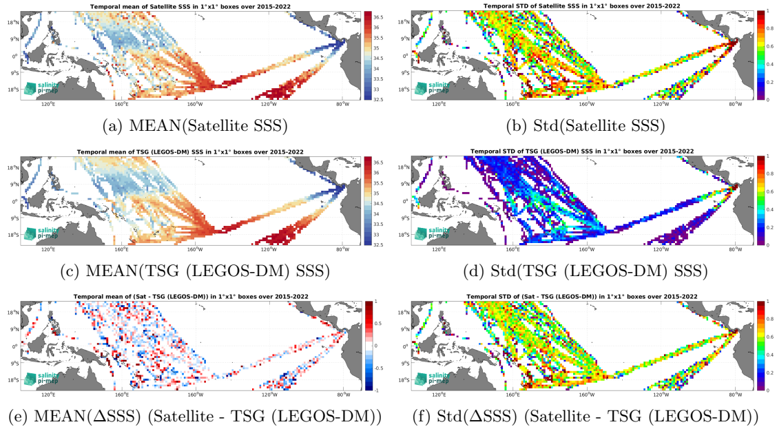
Figure 7: Temporal mean (left) and Std (right) of SSS from SMAP SSS L2 v5.3 - 40 km (RSS) (top), TSG (LEGOS-DM) (middle), and of \Delta SSS (Satellite - TSG (LEGOS-DM)). Only match-up pairs are used to generate these maps.
