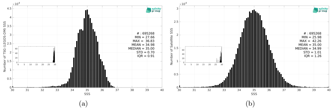
Figure 3: Histograms of SSS from TSG (LEGOS-DM) (a) and SMAP SSS L2 v5.3 - 40 km (RSS) (b) considering all match-up pairs per bins of 0.1 over the Tropical Pacific Ocean Pi-MEP region and for the full satellite product period.
