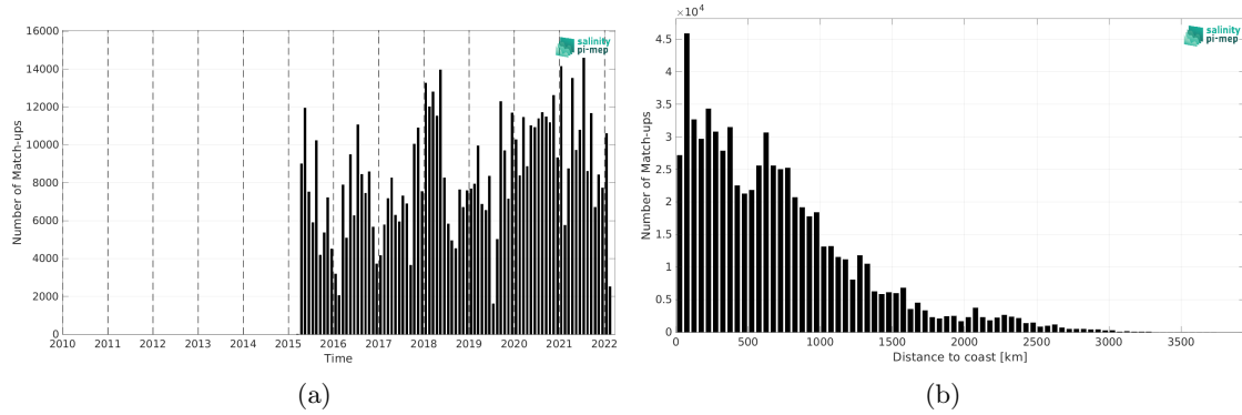
Figure 2: Number of match-ups between TSG (LEGOS-DM) and SMAP SSS L2 v5.3 - 40 km (RSS) SSS as a function of time (a) and as function of the distance to coast (b) over the Tropical Pacific Ocean Pi-MEP region and for the full satellite product period.
