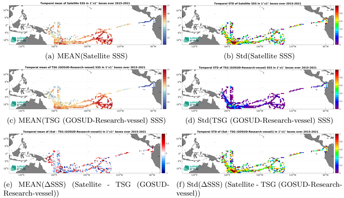
Figure 7: Temporal mean (left) and Std (right) of SSS from SMAP SSS L2 v5.3 - 40 km (RSS) (top), TSG (GOSUD-Research-vessel) (middle), and of \Delta SSS (Satellite - TSG (GOSUD-Research-vessel)). Only match-up pairs are used to generate these maps.
