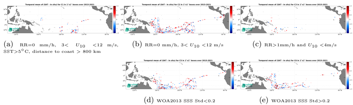
Figure 14: Temporal mean gridded over spatial boxes of size 1^\circ \times 1^\circ of \Delta SSS (SMAP SSS L2 v5.3 - 40 km (RSS) - TSG (GOSUD-Research-vessel)) for 5 different subdatasets corresponding to: RR=0 mm/h, 3 < U_{10} < 12 m/s, SST > 5^\circ\text{C} , distance to coast > 800 km (a), RR=0 mm/h, 3 < U_{10} < 12 m/s (b), RR > 1 mm/h and U_{10} < 4 m/s (c), WOA2013 SSS Std < 0.2 (d), WOA2013 SSS Std > 0.2 (e).
