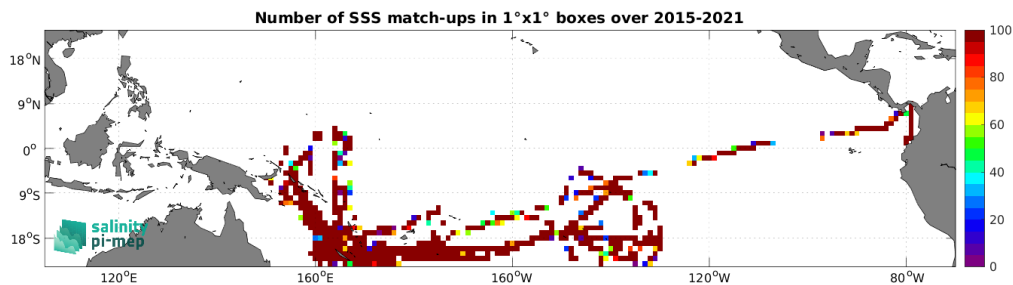
Figure 5: Number of SSS match-ups between TSG (GOSUD-Research-vessel) SSS and the SMAP SSS L2 v5.3 - 40 km (RSS) SSS product for the Tropical Pacific Ocean Pi-MEP region over 1^\circ \times 1^\circ boxes and for the full satellite product period.
