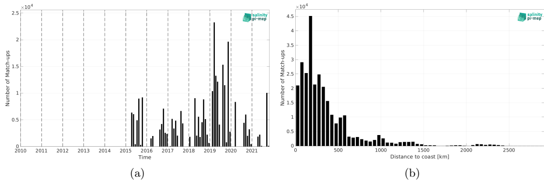
Figure 2: Number of match-ups between TSG (GOSUD-Research-vessel) and SMAP SSS L2 v5.3 - 40 km (RSS) SSS as a function of time (a) and as function of the distance to coast (b) over the Tropical Pacific Ocean Pi-MEP region and for the full satellite product period.
