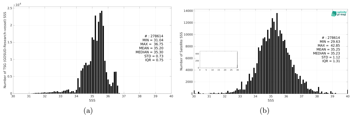
Figure 3: Histograms of SSS from TSG (GOSUD-Research-vessel) (a) and SMAP SSS L2 v5.3 - 40 km (RSS) (b) considering all match-up pairs per bins of 0.1 over the Tropical Pacific Ocean Pi-MEP region and for the full satellite product period.
