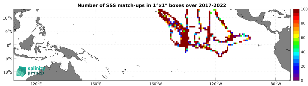
Figure 5: Number of SSS match-ups between Saildrone SSS and the SMAP SSS L2 v5.3 - 40 km (RSS) SSS product for the Tropical Pacific Ocean Pi-MEP region over 1^\circ \times 1^\circ boxes and for the full satellite product period.
