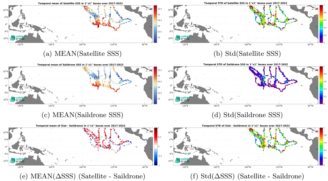
Figure 7: Temporal mean (left) and Std (right) of SSS from SMAP SSS L2 v5.3 - 40 km (RSS) (top), Saildrone (middle), and of \Delta SSS (Satellite - Saildrone). Only match-up pairs are used to generate these maps.
