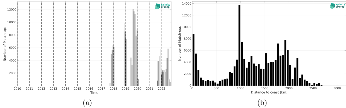
Figure 2: Number of match-ups between Saildrone and SMAP SSS L2 v5.3 - 40 km (RSS) SSS as a function of time (a) and as function of the distance to coast (b) over the Tropical Pacific Ocean Pi-MEP region and for the full satellite product period.
