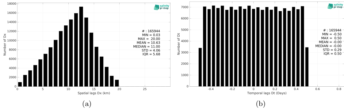
Figure 6: Histograms of the spatial (a) and temporal (b) lags between the location/time of the Sairdron measurement and the date of the corresponding SMAP SSS L2 v5.3 - 40 km (RSS) SSS pixel.
