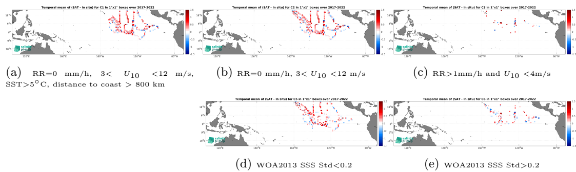
Figure 14: Temporal mean gridded over spatial boxes of size 1^\circ \times 1^\circ of \Delta SSS (SMAP SSS L2 v5.3 - 40 km (RSS) - Sairdron) for 5 different subdatasets corresponding to: RR=0 mm/h, 3 < U_{10} < 12 m/s, SST > 5^\circ C , distance to coast > 800 km (a), RR=0 mm/h, 3 < U_{10} < 12 m/s (b), RR > 1 mm/h and U_{10} < 4 m/s (c), WOA2013 SSS Std < 0.2 (d), WOA2013 SSS Std > 0.2 (e).
