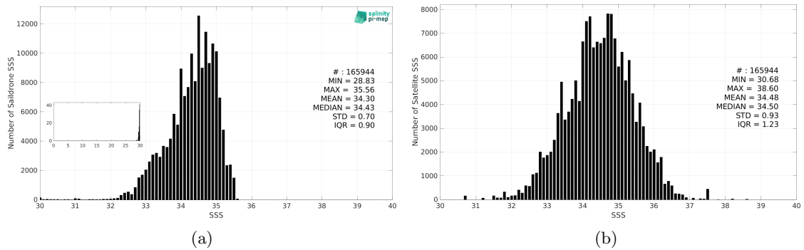
Figure 3: Histograms of SSS from Saildrone (a) and SMAP SSS L2 v5.3 - 40 km (RSS) (b) considering all match-up pairs per bins of 0.1 over the Tropical Pacific Ocean Pi-MEP region and for the full satellite product period.
