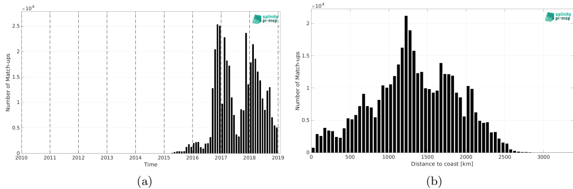
Figure 2: Number of match-ups between Surface drifters and SMAP SSS L2 v5.3 - 40 km (RSS) SSS as a function of time (a) and as function of the distance to coast (b) over the Tropical Pacific Ocean Pi-MEP region and for the full satellite product period.
