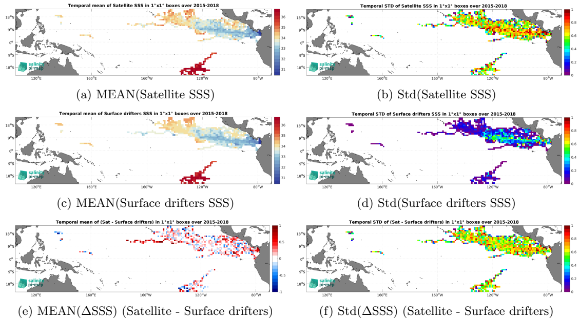
Figure 6: Temporal mean (left) and Std (right) of SSS from SMAP SSS L2 v5.3 - 40 km (RSS) (top), Surface drifters (middle), and of \Delta SSS (Satellite - Surface drifters). Only match-up pairs are used to generate these maps.
