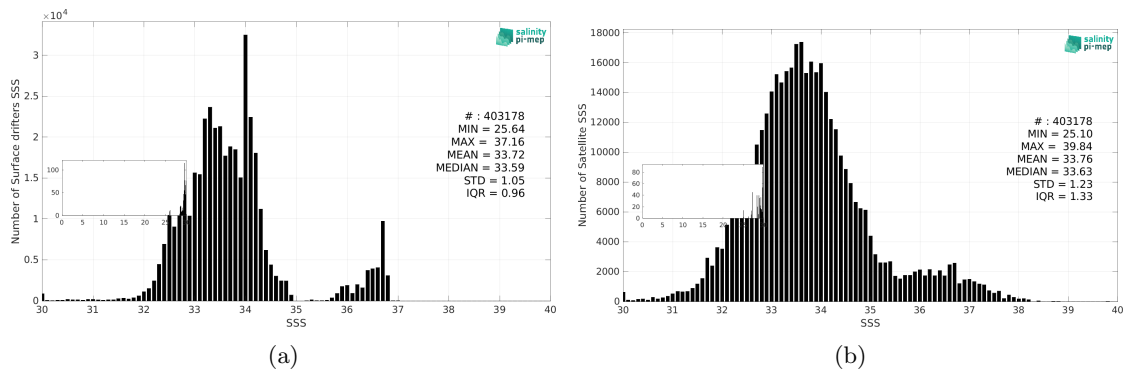
Figure 3: Histograms of SSS from Surface drifters (a) and SMAP SSS L2 v5.3 - 40 km (RSS) (b) considering all match-up pairs per bins of 0.1 over the Tropical Pacific Ocean Pi-MEP region and for the full satellite product period.
