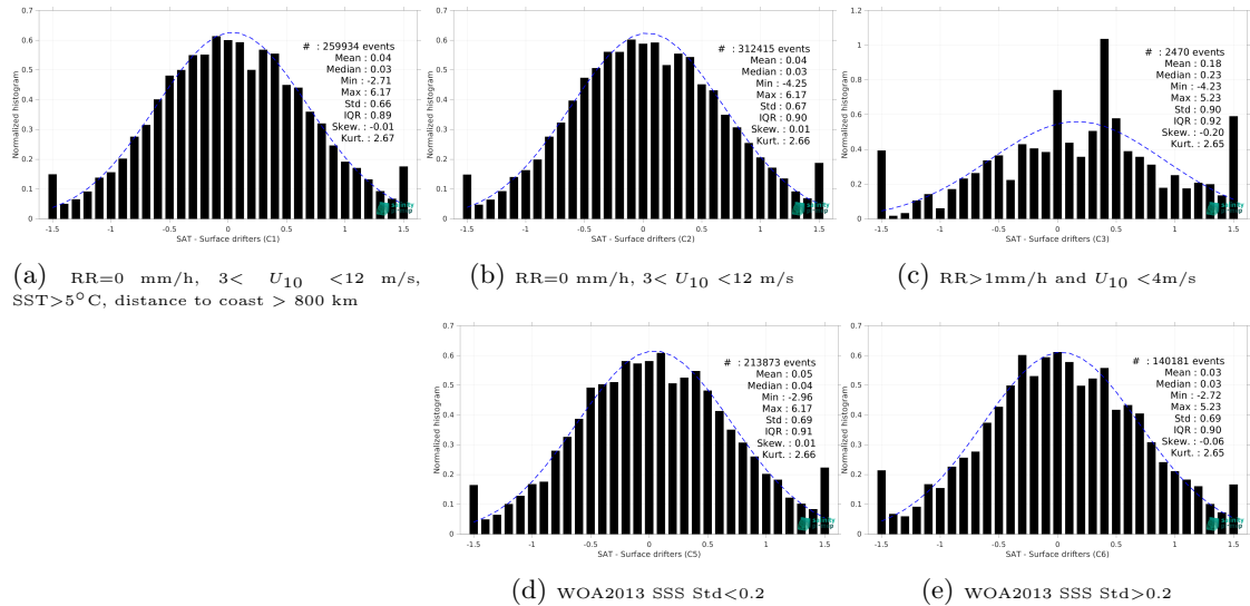
Figure 14: Normalized histogram of \Delta\text{SSS} (SMAP SSS L2 v5.3 - 40 km (RSS) - Surface drifters) for 5 different subdatasets corresponding to: RR=0 mm/h, 3 < U_{10} < 12 m/s, SST >5^\circ\text{C} , distance to coast > 800 km (a), RR=0 mm/h, 3 < U_{10} < 12 m/s (b), RR >1 mm/h and U_{10} < 4 m/s (c), WOA2013 SSS Std <0.2 (d), WOA2013 SSS Std >0.2 (e).
