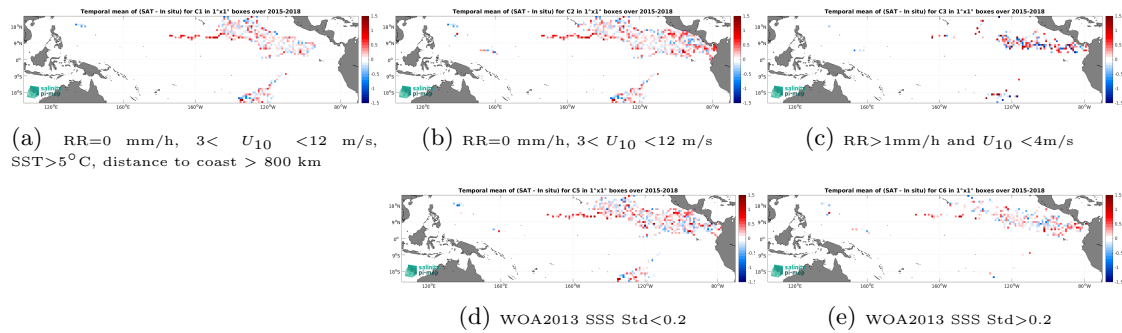
Figure 13: Temporal mean gridded over spatial boxes of size 1^\circ \times 1^\circ of \Delta\text{SSS} (SMAP SSS L2 v5.3 - 40 km (RSS) - Surface drifters) for 5 different subdatasets corresponding to:RR=0 mm/h, 3 < U_{10} < 12 m/s, SST >5^\circ\text{C} , distance to coast > 800 km (a), RR=0 mm/h, 3 < U_{10} < 12 m/s (b), RR >1 mm/h and U_{10} < 4 m/s (c), WOA2013 SSS Std <0.2 (d), WOA2013 SSS Std >0.2 (e).
