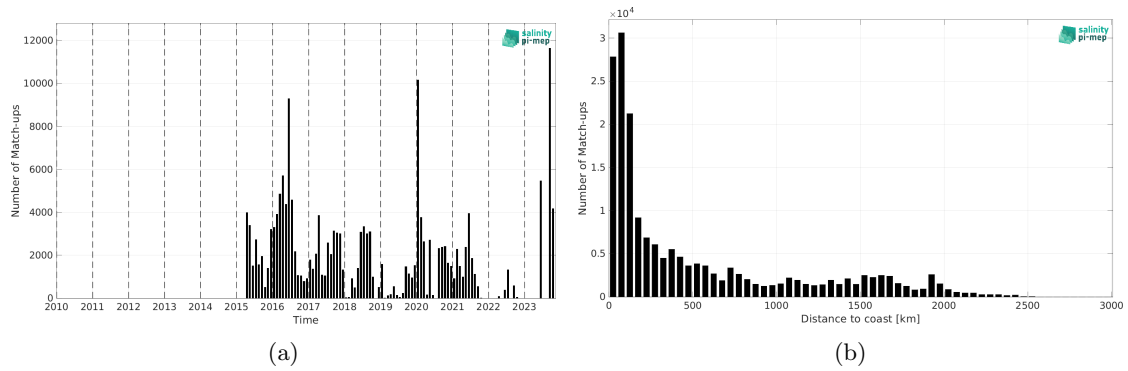
Figure 1: Number of match-ups between TSG (SAMOS) and SMAP SSS L2 v5 - 40 km (RSS) SSS as a function of time (a) and as function of the distance to coast (b) over the Tropical Pacific Ocean Pi-MEP region and for the full satellite product period.
