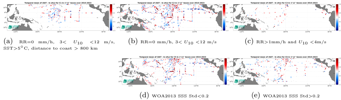
Figure 12: Temporal mean gridded over spatial boxes of size 1^\circ \times 1^\circ of \Delta\text{SSS} (SMAP SSS L2 v5 - 40 km (RSS) - TSG (SAMOS)) for 5 different subdatasets corresponding to:RR=0 mm/h, 3 < U_{10} < 12 m/s, SST >5^\circ\text{C} , distance to coast > 800 km (a), RR=0 mm/h, 3 < U_{10} < 12 m/s (b), RR >1 mm/h and U_{10} < 4 m/s (c), WOA2013 SSS Std <0.2 (d), WOA2013 SSS Std >0.2 (e).
