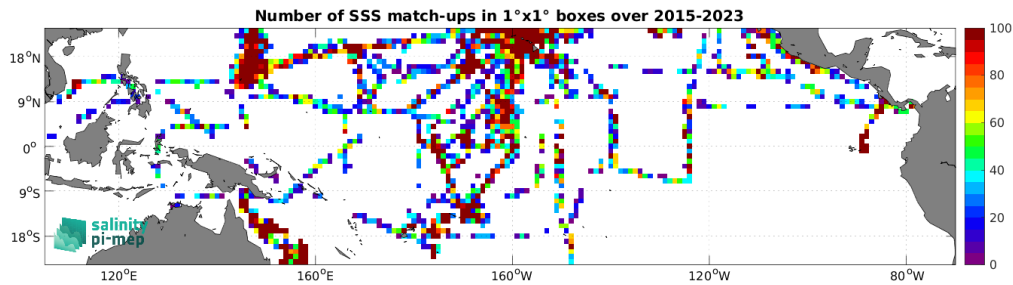
Figure 4: Number of SSS match-ups between TSG (SAMOS) SSS and the SMAP SSS L2 v5 - 40 km (RSS) SSS product for the Tropical Pacific Ocean Pi-MEP region over 1^\circ \times 1^\circ boxes and for the full satellite product period.
