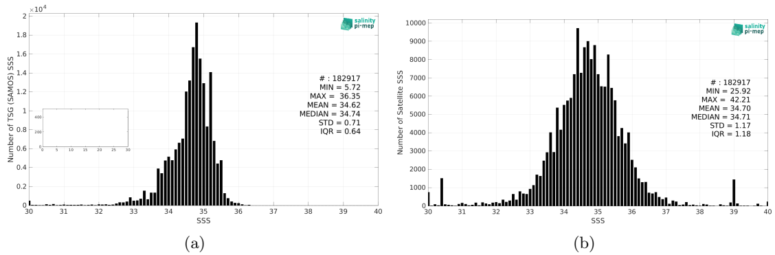
Figure 2: Histograms of SSS from TSG (SAMOS) (a) and SMAP SSS L2 v5 - 40 km (RSS) (b) considering all match-up pairs per bins of 0.1 over the Tropical Pacific Ocean Pi-MEP region and for the full satellite product period.
