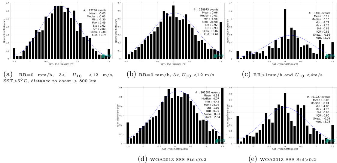
Figure 13: Normalized histogram of \Delta\text{SSS} (SMAP SSS L2 v5 - 40 km (RSS) - TSG (SAMOS)) for 5 different subdatasets corresponding to: RR=0 mm/h, 3 < U_{10} < 12 m/s, SST >5^\circ\text{C} , distance to coast > 800 km (a), RR=0 mm/h, 3 < U_{10} < 12 m/s (b), RR >1 mm/h and U_{10} < 4 m/s (c), WOA2013 SSS Std <0.2 (d), WOA2013 SSS Std >0.2 (e).
