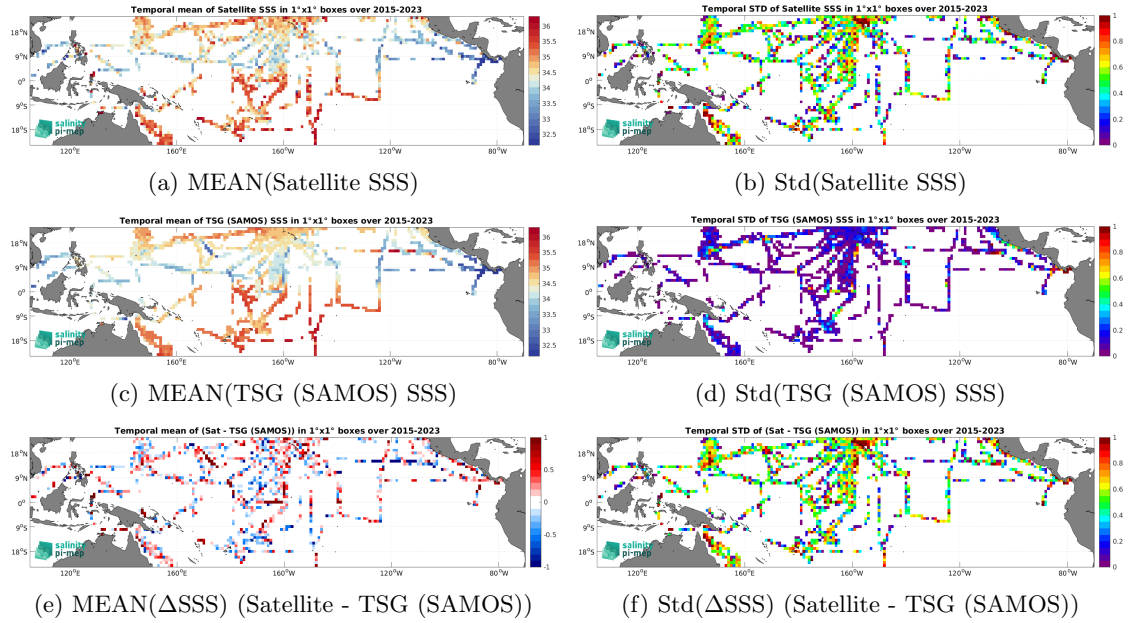
Figure 6: Temporal mean (left) and Std (right) of SSS from SMAP SSS L2 v5 - 40 km (RSS) (top), TSG (SAMOS) (middle), and of \Delta SSS (Satellite - TSG (SAMOS)). Only match-up pairs are used to generate these maps.
