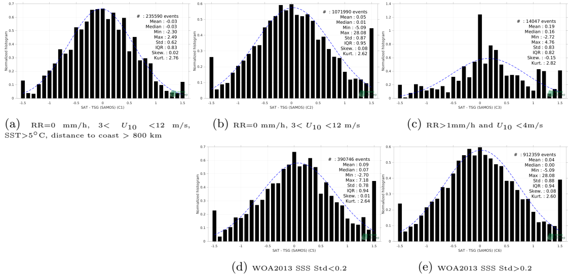
Figure 13: Normalized histogram of \Delta SSS (SMAP SSS L2 v5 - 40 km (RSS) - TSG (SAMOS)) for 5 different subdatasets corresponding to: RR=0 mm/h, 3 < U_{10} < 12 m/s, SST > 5^\circ C , distance to coast > 800 km (a), RR=0 mm/h, 3 < U_{10} < 12 m/s (b), RR > 1\text{mm/h} and U_{10} < 4\text{m/s} (c), WOA2013 SSS Std<0.2 (d), WOA2013 SSS Std>0.2 (e).
