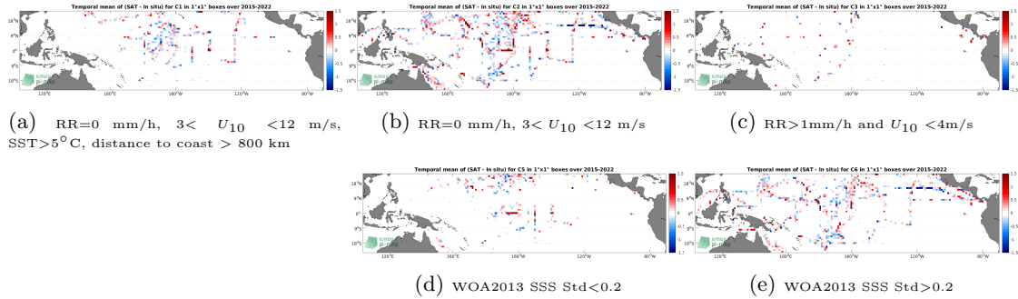
Figure 12: Temporal mean gridded over spatial boxes of size 1^\circ \times 1^\circ of \Delta SSS (SMAP SSS L2 v5 - 40 km (RSS) - TSG (SAMOS)) for 5 different subdatasets corresponding to:RR=0 mm/h, 3 < U_{10} < 12 m/s, SST > 5^\circ C , distance to coast > 800 km (a), RR=0 mm/h, 3 < U_{10} < 12 m/s (b), RR > 1\text{mm/h} and U_{10} < 4\text{m/s} (c), WOA2013 SSS Std<0.2 (d), WOA2013 SSS Std>0.2 (e).
