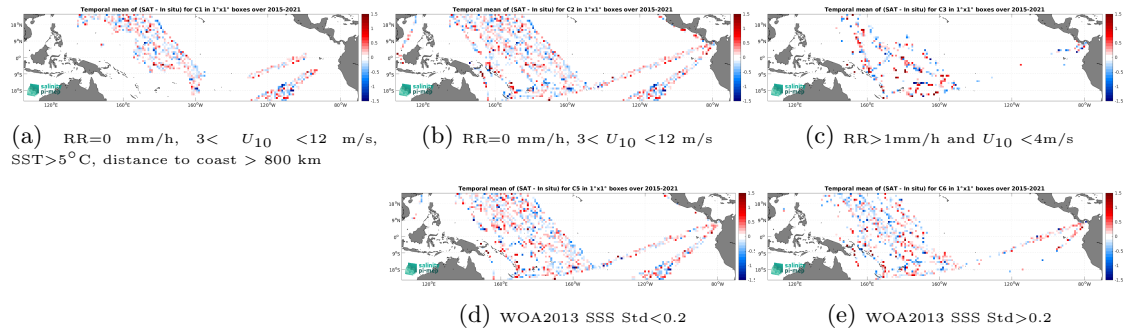
Figure 12: Temporal mean gridded over spatial boxes of size 1^\circ \times 1^\circ of \Delta\text{SSS} (SMAP SSS L2 v5 - 40 km (RSS) - TSG (LEGOS-DM)) for 5 different subdatasets corresponding to:RR=0 mm/h, 3 < U_{10} < 12 m/s, \text{SST} > 5^\circ\text{C} , distance to coast > 800 km (a), RR=0 mm/h, 3 < U_{10} < 12 m/s (b), RR >1 mm/h and U_{10} < 4 m/s (c), WOA2013 SSS Std <0.2 (d), WOA2013 SSS Std >0.2 (e).
