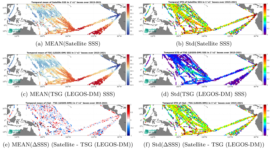
Figure 6: Temporal mean (left) and Std (right) of SSS from SMAP SSS L2 v5 - 40 km (RSS) (top), TSG (LEGOS-DM) (middle), and of \Delta SSS (Satellite - TSG (LEGOS-DM)). Only match-up pairs are used to generate these maps.
