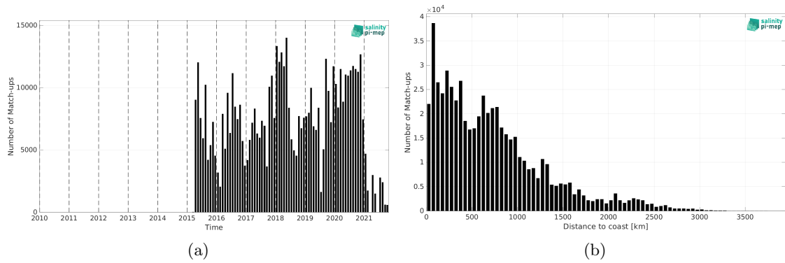
Figure 1: Number of match-ups between TSG (LEGOS-DM) and SMAP SSS L2 v5 - 40 km (RSS) SSS as a function of time (a) and as function of the distance to coast (b) over the Tropical Pacific Ocean Pi-MEP region and for the full satellite product period.
