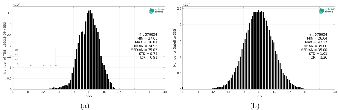
Figure 2: Histograms of SSS from TSG (LEGOS-DM) (a) and SMAP SSS L2 v5 - 40 km (RSS) (b) considering all match-up pairs per bins of 0.1 over the Tropical Pacific Ocean Pi-MEP region and for the full satellite product period.
