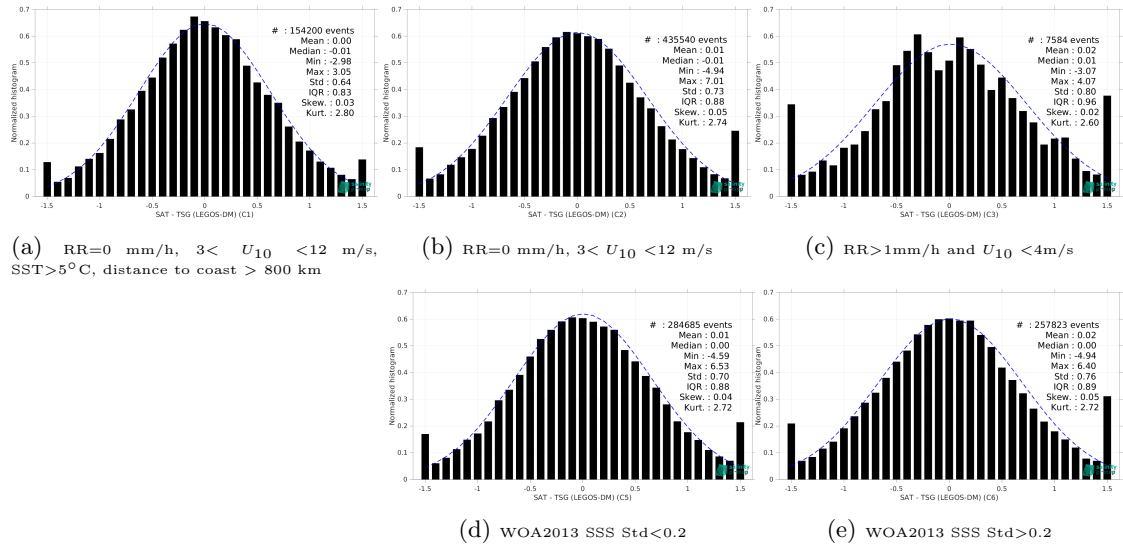
Figure 13: Normalized histogram of \Delta\text{SSS} (SMAP SSS L2 v5 - 40 km (RSS) - TSG (LEGOS-DM)) for 5 different subdatasets corresponding to: RR=0 mm/h, 3 < U_{10} < 12 m/s, \text{SST} > 5^\circ\text{C} , distance to coast > 800 km (a), RR=0 mm/h, 3 < U_{10} < 12 m/s (b), RR >1 mm/h and U_{10} < 4 m/s (c), WOA2013 SSS Std <0.2 (d), WOA2013 SSS Std >0.2 (e).
