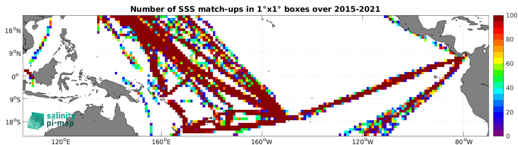
Figure 4: Number of SSS match-ups between TSG (LEGOS-DM) SSS and the SMAP SSS L2 v5 - 40 km (RSS) SSS product for the Tropical Pacific Ocean Pi-MEP region over 1^\circ \times 1^\circ boxes and for the full satellite product period.
