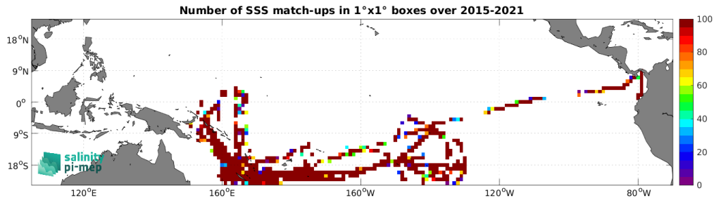
Figure 4: Number of SSS match-ups between TSG (GOSUD-Research-vessel) SSS and the SMAP SSS L2 v5 - 40 km (RSS) SSS product for the Tropical Pacific Ocean Pi-MEP region over 1^\circ \times 1^\circ boxes and for the full satellite product period.
