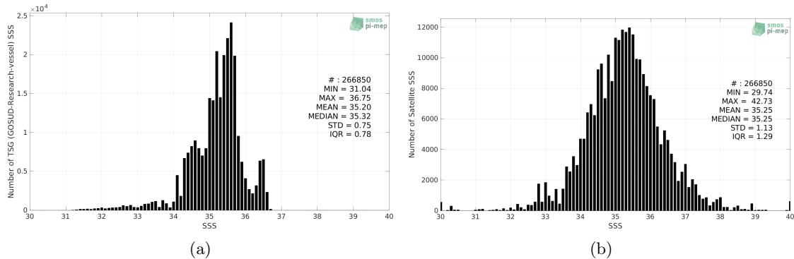
Figure 2: Histograms of SSS from TSG (GOSUD-Research-vessel) (a) and SMAP SSS L2 v5 - 40 km (RSS) (b) considering all match-up pairs per bins of 0.1 over the Tropical Pacific Ocean Pi-MEP region and for the full satellite product period.
