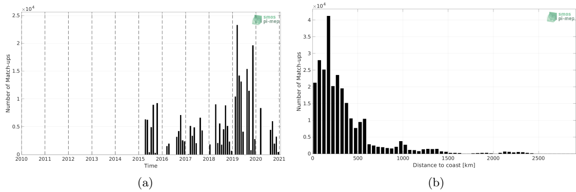
Figure 1: Number of match-ups between TSG (GOSUD-Research-vessel) and SMAP SSS L2 v5 - 40 km (RSS) SSS as a function of time (a) and as function of the distance to coast (b) over the Tropical Pacific Ocean Pi-MEP region and for the full satellite product period.
