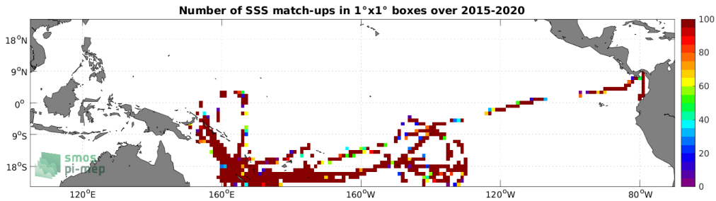
Figure 4: Number of SSS match-ups between TSG (GOSUD-Research-vessel) SSS and the SMAP SSS L2 v5 - 40 km (RSS) SSS product for the Tropical Pacific Ocean Pi-MEP region over 1^\circ \times 1^\circ boxes and for the full satellite product period.
