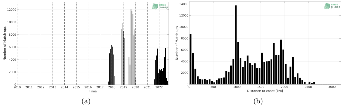
Figure 1: Number of match-ups between Sairdrone and SMAP SSS L2 v5 - 40 km (RSS) SSS as a function of time (a) and as function of the distance to coast (b) over the Tropical Pacific Ocean Pi-MEP region and for the full satellite product period.
