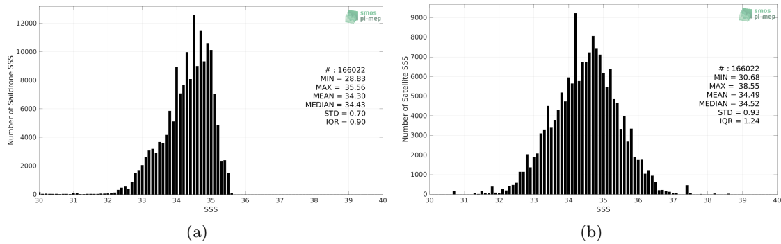
Figure 2: Histograms of SSS from Sairdrone (a) and SMAP SSS L2 v5 - 40 km (RSS) (b) considering all match-up pairs per bins of 0.1 over the Tropical Pacific Ocean Pi-MEP region and for the full satellite product period.
