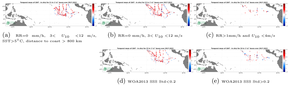
Figure 12: Temporal mean gridded over spatial boxes of size 1^\circ \times 1^\circ of \Delta SSS (SMAP SSS L2 v5 - 40 km (RSS) - Saldrone) for 5 different subdatasets corresponding to:RR=0 mm/h, 3 < U_{10} < 12 m/s, SST >5^\circ C, distance to coast > 800 km (a), RR=0 mm/h, 3 < U_{10} < 12 m/s (b), RR >1 mm/h and U_{10} < 4 m/s (c), WOA2013 SSS Std <0.2 (d), WOA2013 SSS Std >0.2 (e).
