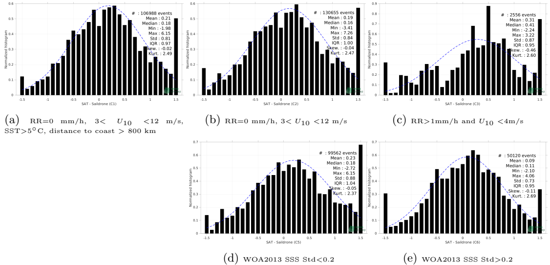
Figure 13: Normalized histogram of \Delta SSS (SMAP SSS L2 v5 - 40 km (RSS) - Saldrone) for 5 different subdatasets corresponding to: RR=0 mm/h, 3 < U_{10} < 12 m/s, SST >5^\circ C, distance to coast > 800 km (a), RR=0 mm/h, 3 < U_{10} < 12 m/s (b), RR >1 mm/h and U_{10} < 4 m/s (c), WOA2013 SSS Std <0.2 (d), WOA2013 SSS Std >0.2 (e).
