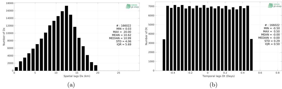
Figure 5: Histograms of the spatial (a) and temporal (b) lags between the location/time of the Sairdrone measurement and the date of the corresponding SMAP SSS L2 v5 - 40 km (RSS) SSS pixel.
