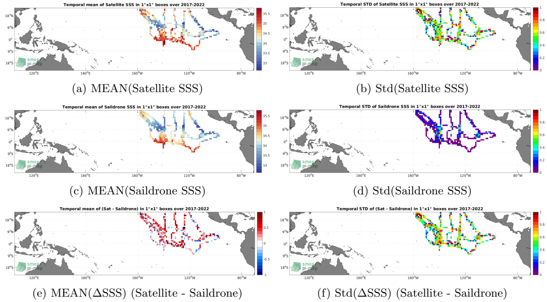
Figure 6: Temporal mean (left) and Std (right) of SSS from SMAP SSS L2 v5 - 40 km (RSS) (top), Saildrone (middle), and of \Delta SSS (Satellite - Saildrone). Only match-up pairs are used to generate these maps.
