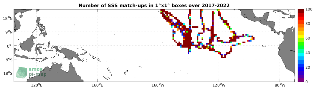
Figure 4: Number of SSS match-ups between Saildrone SSS and the SMAP SSS L2 v5 - 40 km (RSS) SSS product for the Tropical Pacific Ocean Pi-MEP region over 1^\circ \times 1^\circ boxes and for the full satellite product period.
