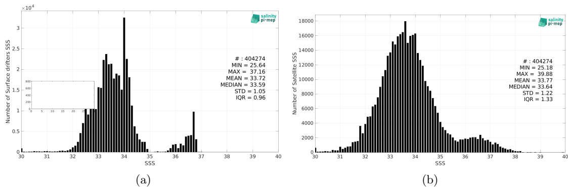
Figure 2: Histograms of SSS from Surface drifters (a) and SMAP SSS L2 v5 - 40 km (RSS) (b) considering all match-up pairs per bins of 0.1 over the Tropical Pacific Ocean Pi-MEP region and for the full satellite product period.
