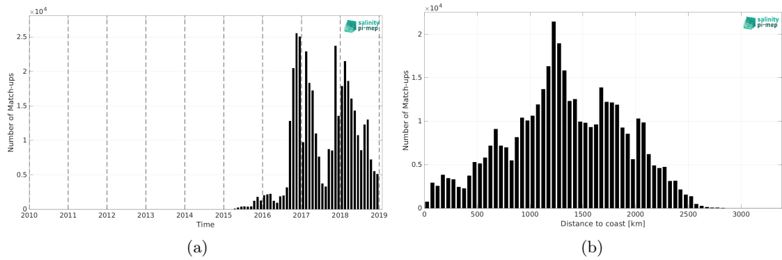
Figure 1: Number of match-ups between Surface drifters and SMAP SSS L2 v5 - 40 km (RSS) SSS as a function of time (a) and as function of the distance to coast (b) over the Tropical Pacific Ocean Pi-MEP region and for the full satellite product period.
