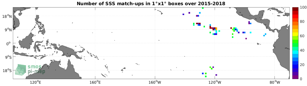
Figure 3: Number of SSS match-ups between Surface drifters SSS and the SMAP SSS L2 v5 - 40 km (RSS) SSS product for the Tropical Pacific Ocean Pi-MEP region over 1^\circ \times 1^\circ boxes and for the full satellite product period.
