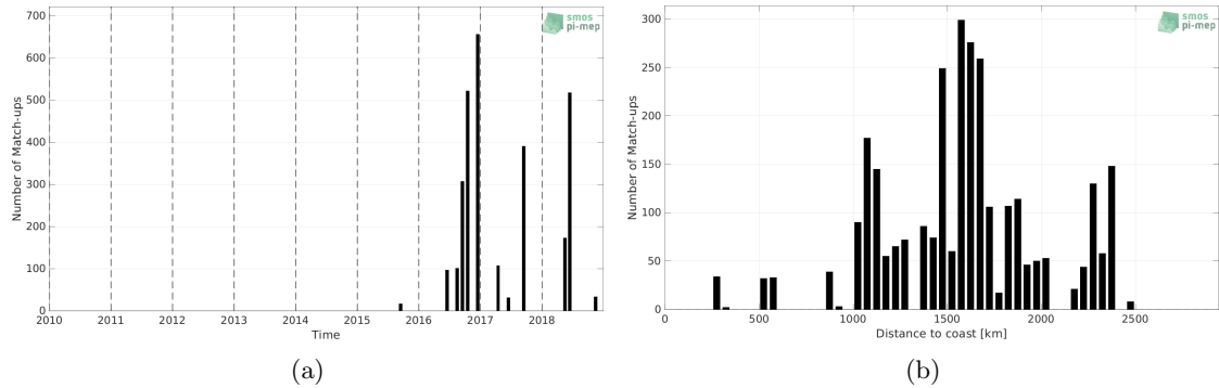
Figure 1: Number of match-ups between Surface drifters and SMAP SSS L2 v5 - 40 km (RSS) SSS as a function of time (a) and as function of the distance to coast (b) over the Tropical Pacific Ocean Pi-MEP region and for the full satellite product period.
