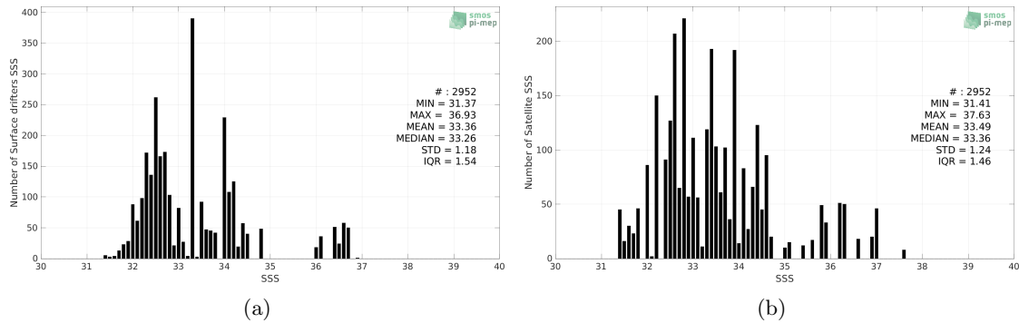
Figure 2: Histograms of SSS from Surface drifters (a) and SMAP SSS L2 v5 - 40 km (RSS) (b) considering all match-up pairs per bins of 0.1 over the Tropical Pacific Ocean Pi-MEP region and for the full satellite product period.
