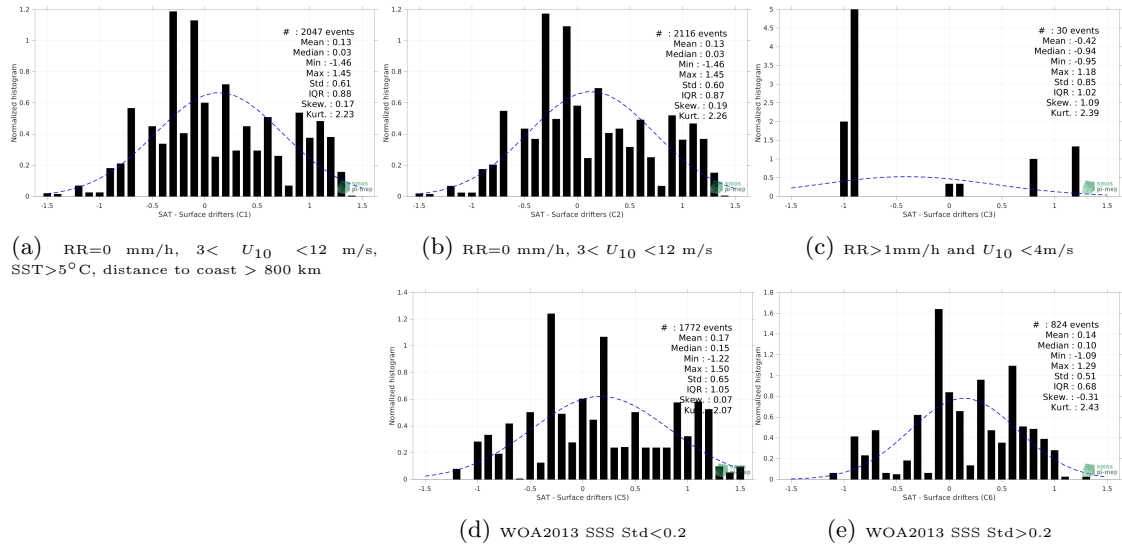
Figure 12: Normalized histogram of \Delta SSS (SMAP SSS L2 v5 - 40 km (RSS) - Surface drifters) for 5 different subdatasets corresponding to: RR=0 mm/h, 3 < U_{10} < 12 m/s, SST > 5^\circ C , distance to coast > 800 km (a), RR=0 mm/h, 3 < U_{10} < 12 m/s (b), RR>1mm/h and U_{10} < 4 m/s (c), WOA2013 SSS Std<0.2 (d), WOA2013 SSS Std>0.2 (e).
