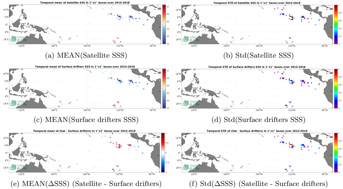
Figure 5: Temporal mean (left) and Std (right) of SSS from SMAP SSS L2 v5 - 40 km (RSS) (top), Surface drifters (middle), and of \Delta SSS (Satellite - Surface drifters). Only match-up pairs are used to generate these maps.
