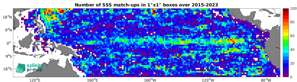
Figure 4: Number of SSS match-ups between Argo SSS and the SMAP SSS L2 v5 - 40 km (RSS) SSS product for the Tropical Pacific Ocean Pi-MEP region over 1^\circ \times 1^\circ boxes and for the full satellite product period.
