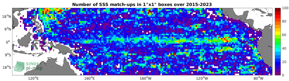
Figure 4: Number of SSS match-ups between Argo SSS and the SMAP SSS L2 v5 - 40 km (RSS) SSS product for the Tropical Pacific Ocean Pi-MEP region over 1^\circ \times 1^\circ boxes and for the full satellite product period.
