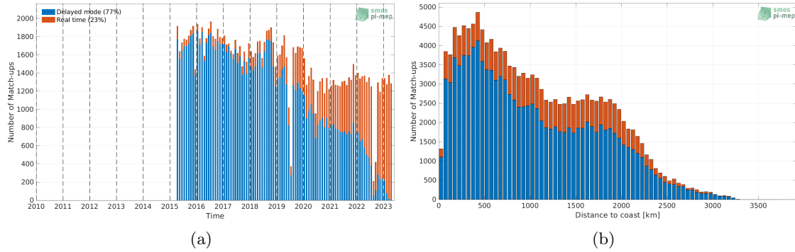
Figure 1: Number of match-ups between Argo and SMAP SSS L2 v5 - 40 km (RSS) SSS as a function of time (a) and as function of the distance to coast (b) over the Tropical Pacific Ocean Pi-MEP region and for the full satellite product period.
