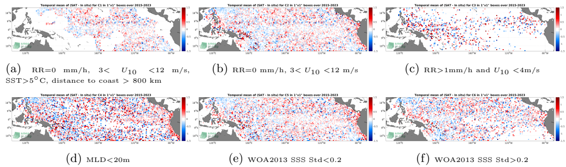
Figure 12: Temporal mean gridded over spatial boxes of size 1^\circ \times 1^\circ of \Delta SSS (SMAP SSS L2 v5 - 40 km (RSS) - Argo) for 6 different subdatasets corresponding to:RR=0 mm/h, 3 < U_{10} < 12 m/s, SST >5^\circ\text{C} , distance to coast > 800 km (a), RR=0 mm/h, 3 < U_{10} < 12 m/s (b), RR >1 mm/h and U_{10} < 4 m/s (c),MLD <20 m (d),WOA2013 SSS Std <0.2 (e),WOA2013 SSS Std >0.2 (f).
