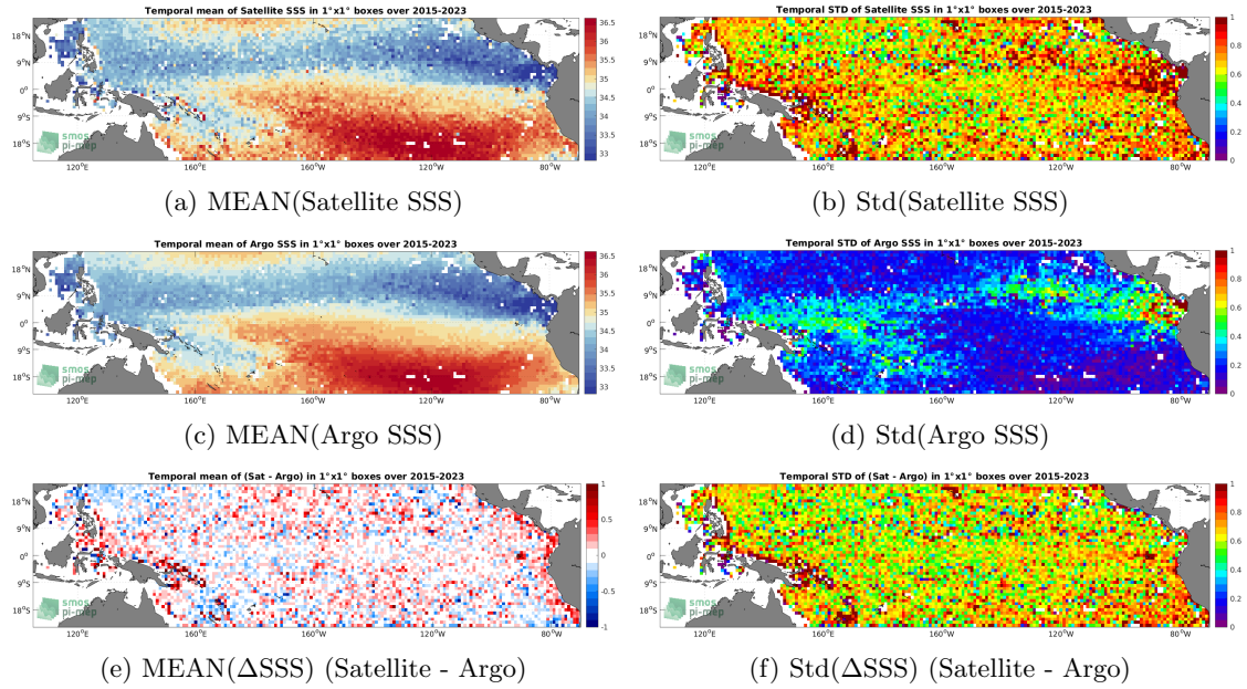
Figure 6: Temporal mean (left) and Std (right) of SSS from SMAP SSS L2 v5 - 40 km (RSS) (top), Argo (middle), and of \Delta SSS (Satellite - Argo). Only match-up pairs are used to generate these maps.
