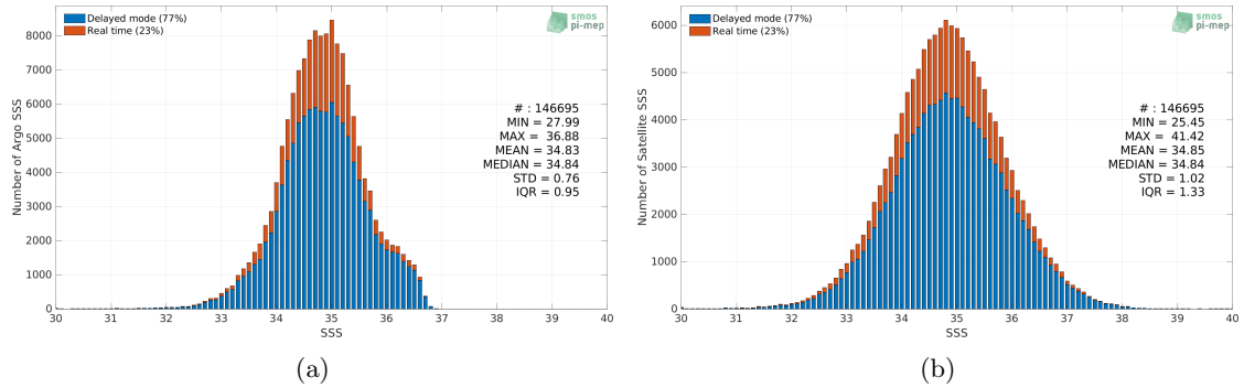
Figure 2: Histograms of SSS from Argo (a) and SMAP SSS L2 v5 - 40 km (RSS) (b) considering all match-up pairs per bins of 0.1 over the Tropical Pacific Ocean Pi-MEP region and for the full satellite product period.
