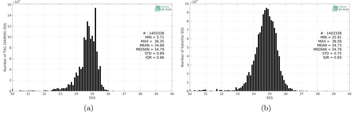
Figure 2: Histograms of SSS from TSG (SAMOS) (a) and SMAP SSS L2 v4 (RSS) (b) considering all match-up pairs per bins of 0.1 over the Tropical Pacific Ocean Pi-MEP region and for the full satellite product period.
