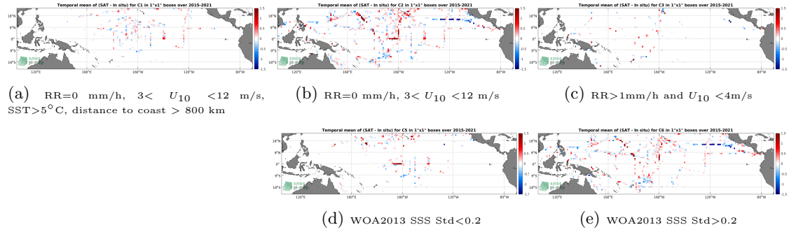
Figure 12: Temporal mean gridded over spatial boxes of size 1^\circ \times 1^\circ of \Delta SSS (SMAP SSS L2 v4 (RSS) - TSG (SAMOS)) for 5 different subdatasets corresponding to: RR=0 mm/h, 3 < U_{10} < 12 m/s, SST > 5^\circ C , distance to coast > 800 km (a), RR=0 mm/h, 3 < U_{10} < 12 m/s (b), RR > 1 mm/h and U_{10} < 4 m/s (c), WOA2013 SSS Std < 0.2 (d), WOA2013 SSS Std > 0.2 (e).
