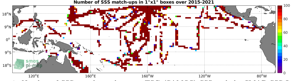
Figure 4: Number of SSS match-ups between TSG (SAMOS) SSS and the SMAP SSS L2 v4 (RSS) SSS product for the Tropical Pacific Ocean Pi-MEP region over 1^\circ \times 1^\circ boxes and for the full satellite product period.
