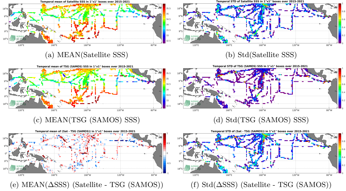
Figure 6: Temporal mean (left) and Std (right) of SSS from SMAP SSS L2 v4 (RSS) (top), TSG (SAMOS) (middle), and of \Delta SSS (Satellite - TSG (SAMOS)). Only match-up pairs are used to generate these maps.
