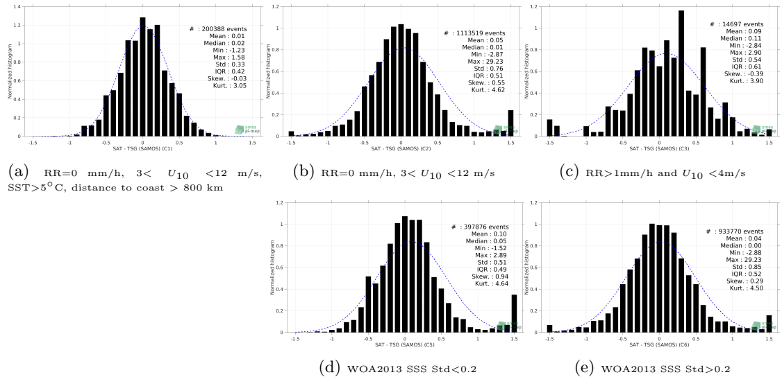
Figure 13: Normalized histogram of \Delta SSS (SMAP SSS L2 v4 (RSS) - TSG (SAMOS)) for 5 different subdatasets corresponding to: RR=0 mm/h, 3 < U_{10} < 12 m/s, SST > 5^\circ C , distance to coast > 800 km (a), RR=0 mm/h, 3 < U_{10} < 12 m/s (b), RR > 1 mm/h and U_{10} < 4 m/s (c), WOA2013 SSS Std < 0.2 (d), WOA2013 SSS Std > 0.2 (e).
