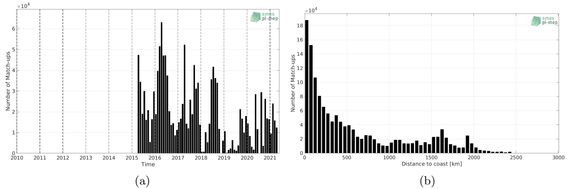
Figure 1: Number of match-ups between TSG (SAMOS) and SMAP SSS L2 v4 (RSS) SSS as a function of time (a) and as function of the distance to coast (b) over the Tropical Pacific Ocean Pi-MEP region and for the full satellite product period.
