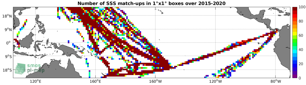
Figure 4: Number of SSS match-ups between TSG (LEGOS-DM) SSS and the SMAP SSS L2 v4 (RSS) SSS product for the Tropical Pacific Ocean Pi-MEP region over 1^\circ \times 1^\circ boxes and for the full satellite product period.
