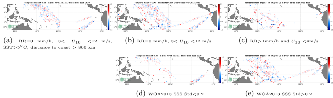
Figure 12: Temporal mean gridded over spatial boxes of size 1°x1° of ΔSSS (SMAP SSS L2 v4 (RSS) - TSG (LEGOS-DM)) for 5 different subdatasets corresponding to: RR=0 mm/h, 3 < U 10 < 12 m/s, SST > 5°C, distance to coast > 800 km (a), RR=0 mm/h, 3 < U 10 < 12 m/s (b), RR > 1mm/h and U 10 < 4m/s (c), WOA2013 SSS Std < 0.2 (d), WOA2013 SSS Std > 0.2 (e).
