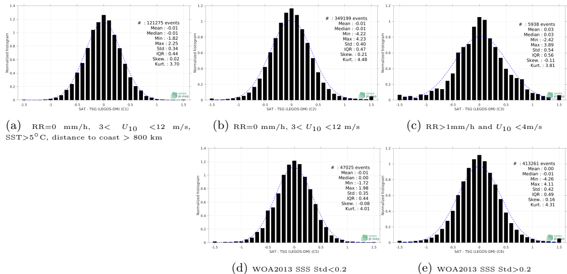
Figure 13: Normalized histogram of ΔSSS (SMAP SSS L2 v4 (RSS) - TSG (LEGOS-DM)) for 5 different subdatasets corresponding to: RR=0 mm/h, 3 < U 10 < 12 m/s, SST > 5°C, distance to coast > 800 km (a), RR=0 mm/h, 3 < U 10 < 12 m/s (b), RR > 1mm/h and U 10 < 4m/s (c), WOA2013 SSS Std < 0.2 (d), WOA2013 SSS Std > 0.2 (e).
