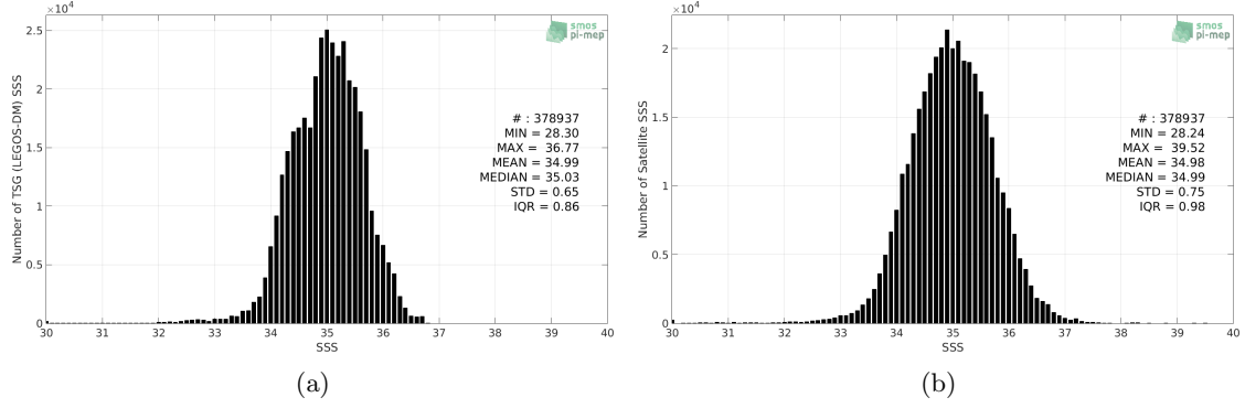
Figure 2: Histograms of SSS from TSG (LEGOS-DM) (a) and SMAP SSS L2 v4 (RSS) (b) considering all match-up pairs per bins of 0.1 over the Tropical Pacific Ocean Pi-MEP region and for the full satellite product period.
