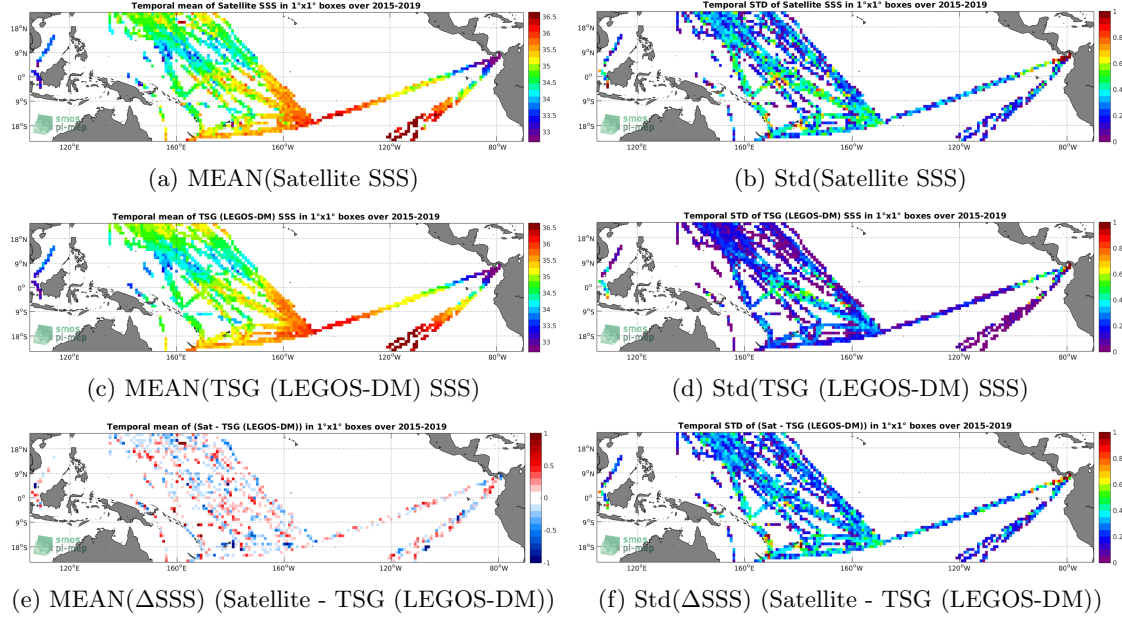
Figure 6: Temporal mean (left) and Std (right) of SSS from SMAP SSS L2 v4 (RSS) (top), TSG (LEGOS-DM) (middle), and of \Delta SSS (Satellite - TSG (LEGOS-DM)). Only match-up pairs are used to generate these maps.
