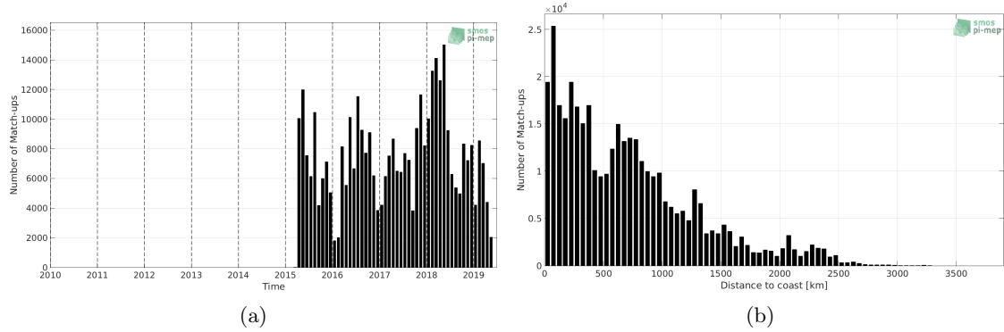
Figure 1: Number of match-ups between TSG (LEGOS-DM) and SMAP SSS L2 v4 (RSS) SSS as a function of time (a) and as function of the distance to coast (b) over the Tropical Pacific Ocean Pi-MEP region and for the full satellite product period.
