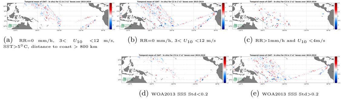
Figure 12: Temporal mean gridded over spatial boxes of size 1^\circ \times 1^\circ of \Delta SSS (SMAP SSS L2 v4 (RSS) - TSG (LEGOS-DM)) for 5 different subdatasets corresponding to: RR=0 mm/h, 3 < U_{10} < 12 m/s, SST > 5^\circ C , distance to coast > 800 km (a), RR=0 mm/h, 3 < U_{10} < 12 m/s (b), RR > 1 mm/h and U_{10} < 4 m/s (c), WOA2013 SSS Std < 0.2 (d), WOA2013 SSS Std > 0.2 (e).
