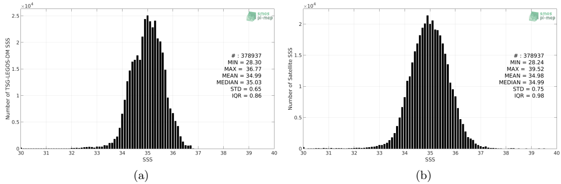
Figure 2: Histograms of SSS from TSG-LEGOS-DM (a) and SMAP-L2-RSS-V4 (b) considering all match-up pairs per bins of 0.1 over the Tropical Pacific Ocean Pi-MEP region and for the full satellite product period.
