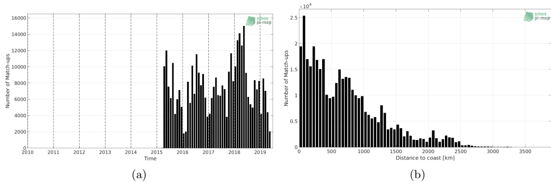
Figure 1: Number of match-ups between TSG-LEGOS-DM and SMAP-L2-RSS-V4 SSS as a function of time (a) and as function of the distance to coast (b) over the Tropical Pacific Ocean Pi-MEP region and for the full satellite product period.
