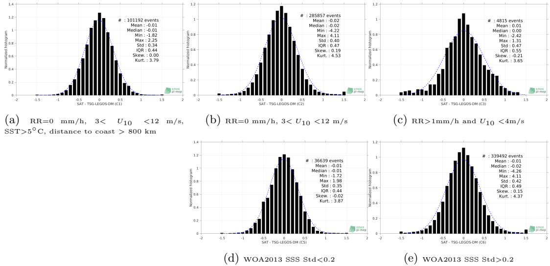
Figure 13: Normalized histogram of \Delta SSS (SMAP-L2-RSS-V4 - TSG-LEGOS-DM) for 5 different subdatasets corresponding to: RR=0 mm/h, 3 < U_{10} < 12 m/s, SST > 5^\circ C , distance to coast > 800 km (a), RR=0 mm/h, 3 < U_{10} < 12 m/s (b), RR > 1 mm/h and U_{10} < 4 m/s (c), WOA2013 SSS Std < 0.2 (d), WOA2013 SSS Std > 0.2 (e).
