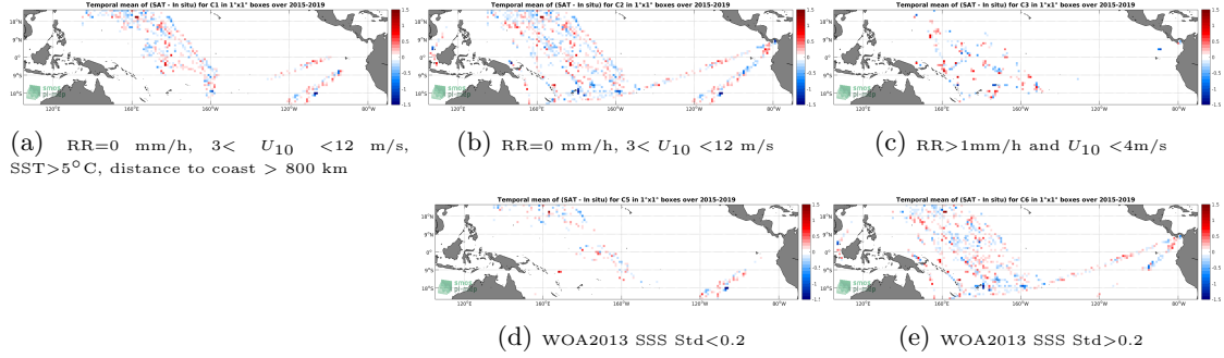
Figure 12: Temporal mean gridded over spatial boxes of size 1^\circ \times 1^\circ of \Delta SSS (SMAP-L2-RSS-V4 - TSG-LEGOS-DM) for 5 different subdatasets corresponding to: RR=0 mm/h, 3 < U_{10} < 12 m/s, SST > 5^\circ C , distance to coast > 800 km (a), RR=0 mm/h, 3 < U_{10} < 12 m/s (b), RR > 1 mm/h and U_{10} < 4 m/s (c), WOA2013 SSS Std < 0.2 (d), WOA2013 SSS Std > 0.2 (e).
