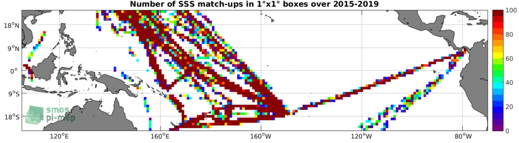
Figure 4: Number of SSS match-ups between TSG-LEGOS-DM SSS and the SMAP-L2-RSS-V4 SSS product for the Tropical Pacific Ocean Pi-MEP region over 1^\circ \times 1^\circ boxes and for the full satellite product period.
