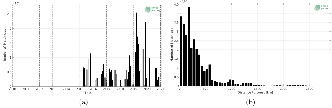
Figure 1: Number of match-ups between TSG (GOSUD-Research-vessel) and SMAP SSS L2 v4 (RSS) SSS as a function of time (a) and as function of the distance to coast (b) over the Tropical Pacific Ocean Pi-MEP region and for the full satellite product period.
