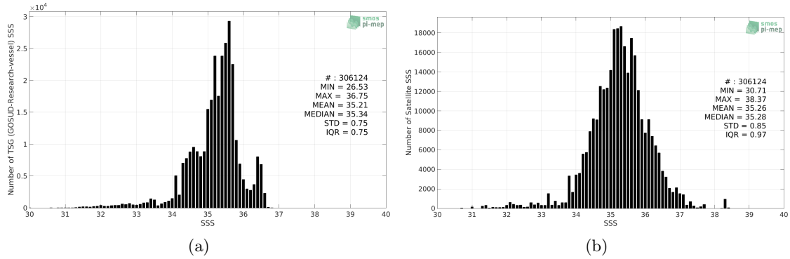
Figure 2: Histograms of SSS from TSG (GOSUD-Research-vessel) (a) and SMAP SSS L2 v4 (RSS) (b) considering all match-up pairs per bins of 0.1 over the Tropical Pacific Ocean Pi-MEP region and for the full satellite product period.
