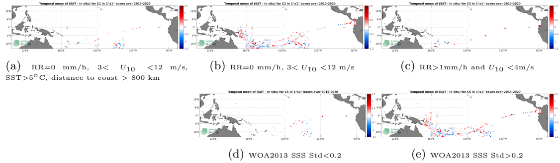
Figure 12: Temporal mean gridded over spatial boxes of size 1^\circ \times 1^\circ of \Delta SSS (SMAP SSS L2 v4 (RSS) - TSG (GOSUD-Research-vessel)) for 5 different subdatasets corresponding to: RR=0 mm/h, 3 < U_{10} < 12 m/s, SST > 5^\circ C , distance to coast > 800 km (a), RR=0 mm/h, 3 < U_{10} < 12 m/s (b), RR > 1 mm/h and U_{10} < 4 m/s (c), WOA2013 SSS Std < 0.2 (d), WOA2013 SSS Std > 0.2 (e).
