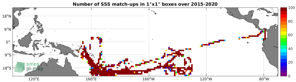
Figure 4: Number of SSS match-ups between TSG (GOSUD-Research-vessel) SSS and the SMAP SSS L2 v4 (RSS) SSS product for the Tropical Pacific Ocean Pi-MEP region over 1^\circ \times 1^\circ boxes and for the full satellite product period.
