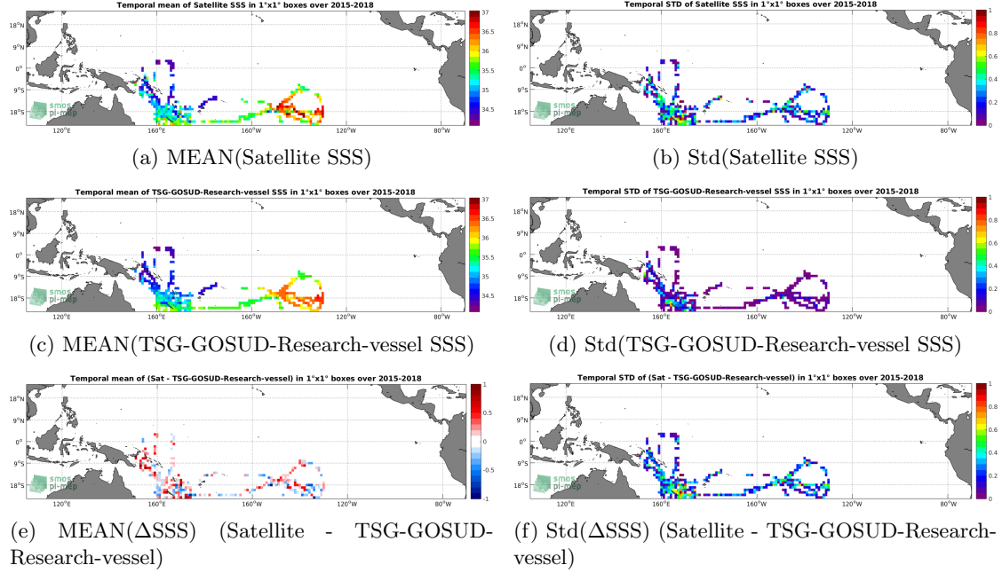
Figure 6: Temporal mean (left) and Std (right) of SSS from SMAP-L2-RSS-V4 (top), TSG-GOSUD-Research-vessel (middle), and of \Delta SSS (Satellite - TSG-GOSUD-Research-vessel). Only match-up pairs are used to generate these maps.
