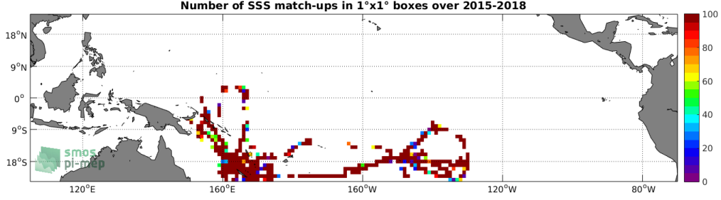
Figure 4: Number of SSS match-ups between TSG-GOSUD-Research-vessel SSS and the SMAP-L2-RSS-V4 SSS product for the Tropical Pacific Ocean Pi-MEP region over 1^\circ \times 1^\circ boxes and for the full satellite product period.
