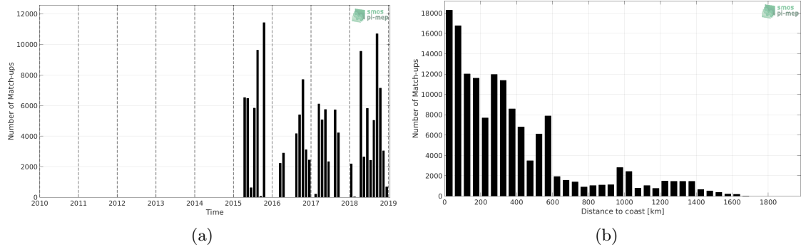
Figure 1: Number of match-ups between TSG-GOSUD-Research-vessel and SMAP-L2-RSS-V4 SSS as a function of time (a) and as function of the distance to coast (b) over the Tropical Pacific Ocean Pi-MEP region and for the full satellite product period.
