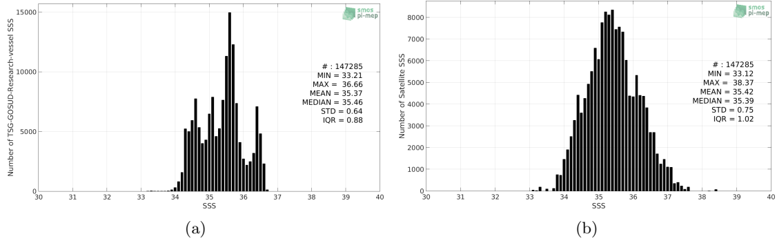
Figure 2: Histograms of SSS from TSG-GOSUD-Research-vessel (a) and SMAP-L2-RSS-V4 (b) considering all match-up pairs per bins of 0.1 over the Tropical Pacific Ocean Pi-MEP region and for the full satellite product period.
