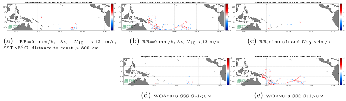
Figure 12: Temporal mean gridded over spatial boxes of size 1^\circ \times 1^\circ of \Delta SSS (SMAP-L2-RSS-V4 - TSG-GOSUD-Research-vessel) for 5 different subdatasets corresponding to: RR=0 mm/h, 3 < U_{10} < 12 m/s, SST > 5^\circ\text{C} , distance to coast > 800 km (a), RR=0 mm/h, 3 < U_{10} < 12 m/s (b), RR > 1 mm/h and U_{10} < 4 m/s (c), WOA2013 SSS Std < 0.2 (d), WOA2013 SSS Std > 0.2 (e).
