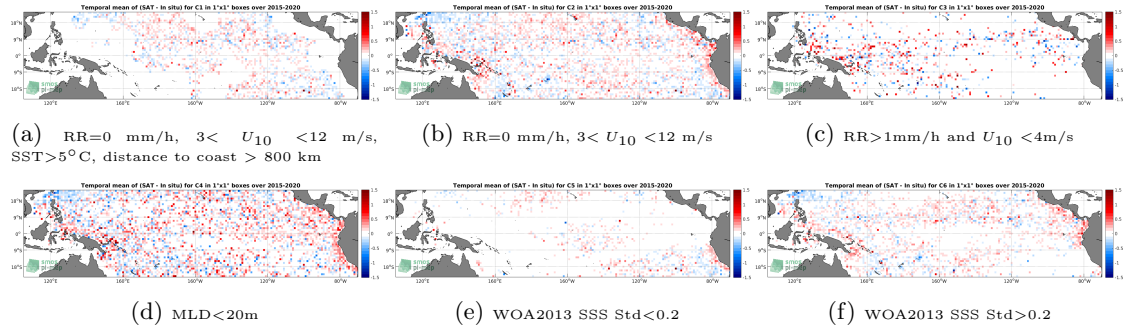
Figure 12: Temporal mean gridded over spatial boxes of size 1^\circ \times 1^\circ of \Delta SSS (SMAP SSS L2 v4 (RSS) - Argo) for 6 different subdatasets corresponding to: RR=0 mm/h, 3 < U_{10} < 12 m/s, SST > 5^\circ C , distance to coast > 800 km (a), RR=0 mm/h, 3 < U_{10} < 12 m/s (b), RR > 1 mm/h and U_{10} < 4 m/s (c), MLD < 20 m (d), WOA2013 SSS Std < 0.2 (e), WOA2013 SSS Std > 0.2 (f).
