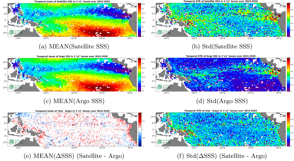
Figure 6: Temporal mean (left) and Std (right) of SSS from SMAP SSS L2 v4 (RSS) (top), Argo (middle), and of \Delta SSS (Satellite - Argo). Only match-up pairs are used to generate these maps.
