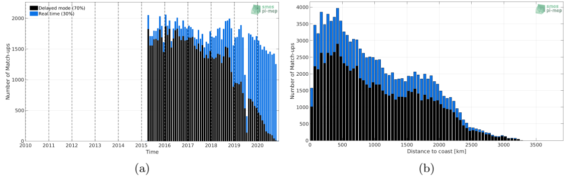
Figure 1: Number of match-ups between Argo and SMAP SSS L2 v4 (RSS) SSS as a function of time (a) and as function of the distance to coast (b) over the Tropical Pacific Ocean Pi-MEP region and for the full satellite product period.
