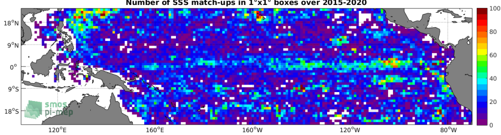
Figure 4: Number of SSS match-ups between Argo SSS and the SMAP SSS L2 v4 (RSS) SSS product for the Tropical Pacific Ocean Pi-MEP region over 1^\circ \times 1^\circ boxes and for the full satellite product period.
