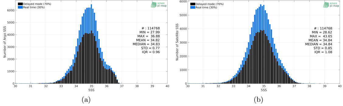
Figure 2: Histograms of SSS from Argo (a) and SMAP SSS L2 v4 (RSS) (b) considering all match-up pairs per bins of 0.1 over the Tropical Pacific Ocean Pi-MEP region and for the full satellite product period.
