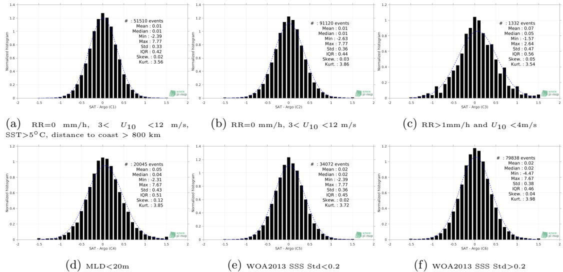
Figure 13: Normalized histogram of \Delta SSS (SMAP SSS L2 v4 (RSS) - Argo) for 6 different subdatasets corresponding to: RR=0 mm/h, 3 < U_{10} < 12 m/s, SST > 5^\circ C , distance to coast > 800 km (a), RR=0 mm/h, 3 < U_{10} < 12 m/s (b), RR > 1 mm/h and U_{10} < 4 m/s (c), MLD < 20 m (d), WOA2013 SSS Std < 0.2 (e), WOA2013 SSS Std > 0.2 (f).
