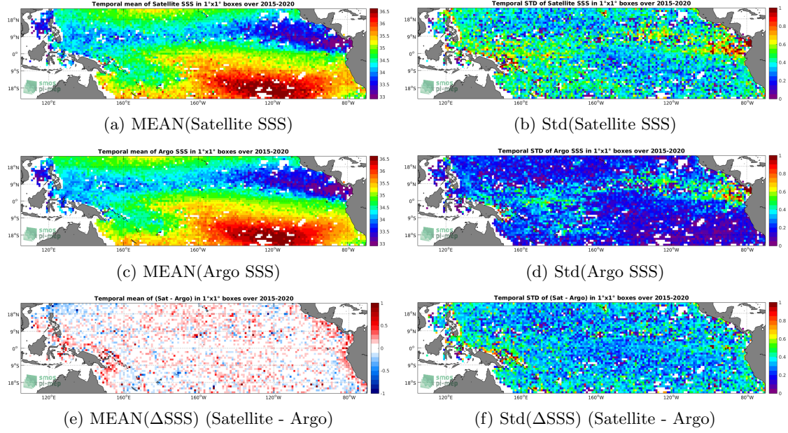
Figure 6: Temporal mean (left) and Std (right) of SSS from SMAP-L2-RSS-V4 (top), Argo (middle), and of \Delta SSS (Satellite - Argo). Only match-up pairs are used to generate these maps.
