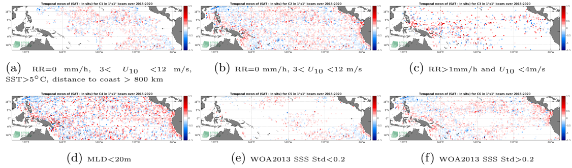
Figure 12: Temporal mean gridded over spatial boxes of size 1^\circ \times 1^\circ of \Delta SSS (SMAP-L2-RSS-V4 - Argo) for 6 different subdatasets corresponding to: RR=0 mm/h, 3 < U_{10} < 12 m/s, SST > 5^\circ C , distance to coast > 800 km (a), RR=0 mm/h, 3 < U_{10} < 12 m/s (b), RR > 1 mm/h and U_{10} < 4 m/s (c), MLD < 20 m (d), WOA2013 SSS Std < 0.2 (e), WOA2013 SSS Std > 0.2 (f).
