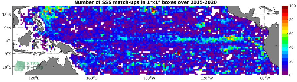
Figure 4: Number of SSS match-ups between Argo SSS and the SMAP-L2-RSS-V4 SSS product for the Tropical Pacific Ocean Pi-MEP region over 1^\circ \times 1^\circ boxes and for the full satellite product period.
