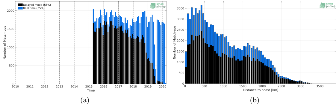
Figure 1: Number of match-ups between Argo and SMAP-L2-RSS-V4 SSS as a function of time (a) and as function of the distance to coast (b) over the Tropical Pacific Ocean Pi-MEP region and for the full satellite product period.
