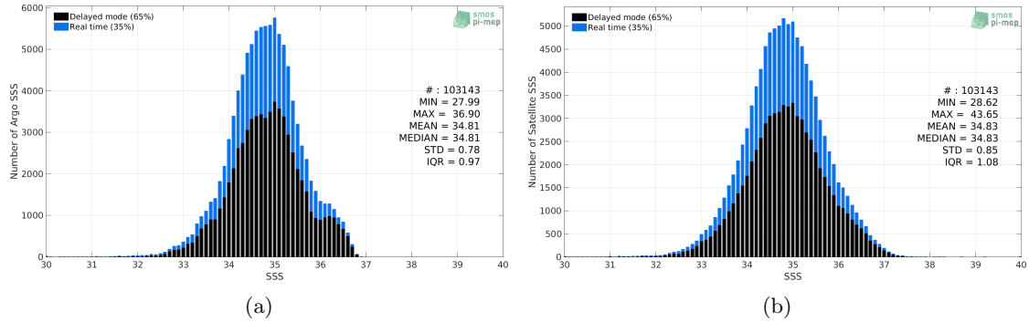
Figure 2: Histograms of SSS from Argo (a) and SMAP-L2-RSS-V4 (b) considering all match-up pairs per bins of 0.1 over the Tropical Pacific Ocean Pi-MEP region and for the full satellite product period.
