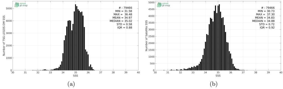
Figure 2: Histograms of SSS from TSG-LEGOS-DM (a) and SMAP-L2-RSS-V3-70KM (b) considering all match-up pairs per bins of 0.1 over the Tropical Pacific Ocean Pi-MEP region and for the full satellite product period.
