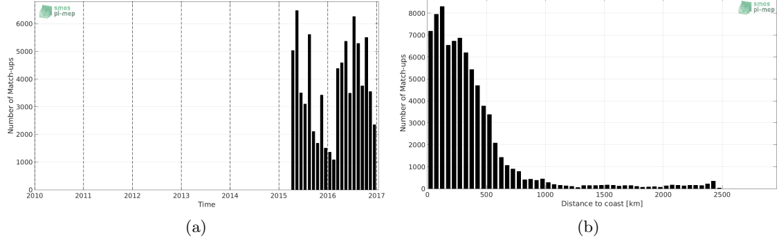
Figure 1: Number of match-ups between TSG-LEGOS-DM and SMAP-L2-RSS-V3-70KM SSS as a function of time (a) and as function of the distance to coast (b) over the Tropical Pacific Ocean Pi-MEP region and for the full satellite product period.
