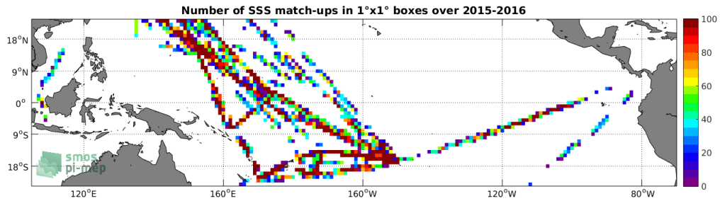
Figure 4: Number of SSS match-ups between TSG-LEGOS-DM SSS and the SMAP-L2-RSS-V3-70KM SSS product for the Tropical Pacific Ocean Pi-MEP region over 1^\circ \times 1^\circ boxes and for the full satellite product period.
