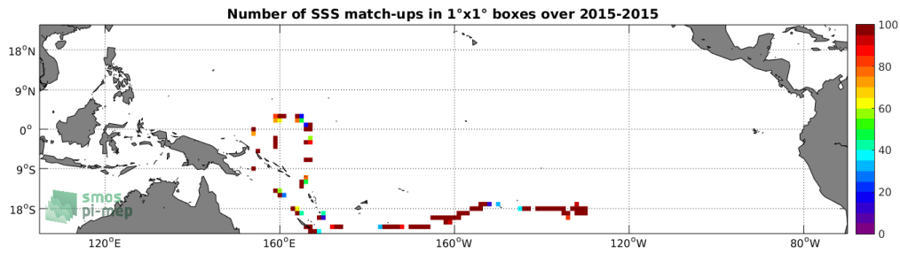
Figure 4: Number of SSS match-ups between TSG-GOSUD-Research-vessel SSS and the SMAP-L2-RSS-V3-70KM SSS product for the Tropical Pacific Ocean Pi-MEP region over 1^\circ \times 1^\circ boxes and for the full satellite product period.
