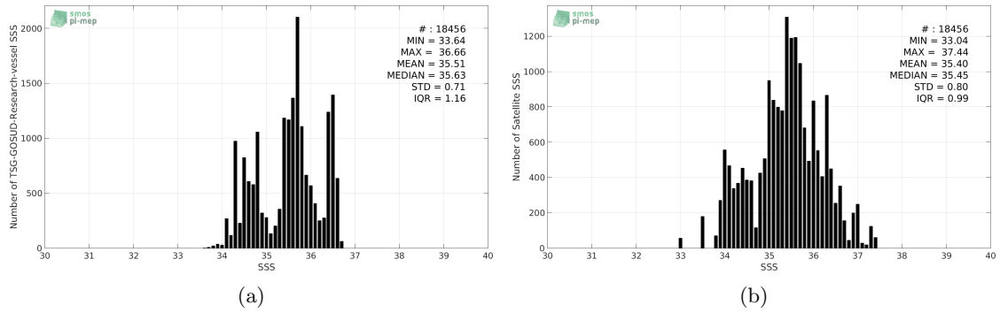
Figure 2: Histograms of SSS from TSG-GOSUD-Research-vessel (a) and SMAP-L2-RSS-V3-70KM (b) considering all match-up pairs per bins of 0.1 over the Tropical Pacific Ocean Pi-MEP region and for the full satellite product period.
