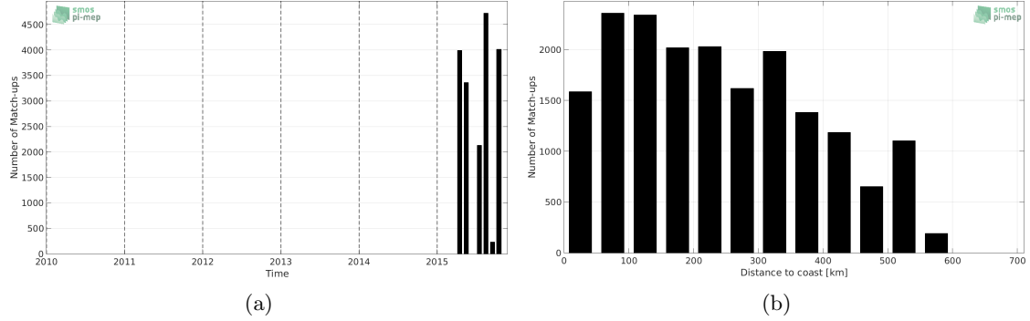
Figure 1: Number of match-ups between TSG-GOSUD-Research-vessel and SMAP-L2-RSS-V3-70KM SSS as a function of time (a) and as function of the distance to coast (b) over the Tropical Pacific Ocean Pi-MEP region and for the full satellite product period.
