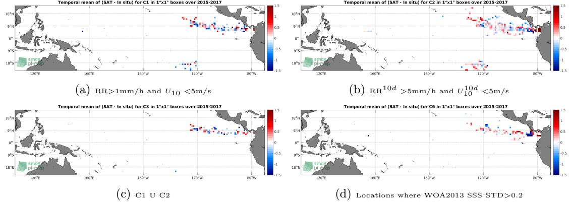
Figure 11: Temporal mean gridded over spatial boxes of size 1^\circ \times 1^\circ of \Delta SSS (SMAP-L2-RSS-V3-70KM - Surface drifters) for 4 different subdatasets corresponding to: RR > 1mm/h and U_{10} < 5\text{m/s} (a), RR^{10d} > 5\text{mm/h} and U_{10}^{10d} < 5\text{m/s} (b), C1 U C2 (c), Locations where WOA2013 SSS STD > 0.2 (d).
