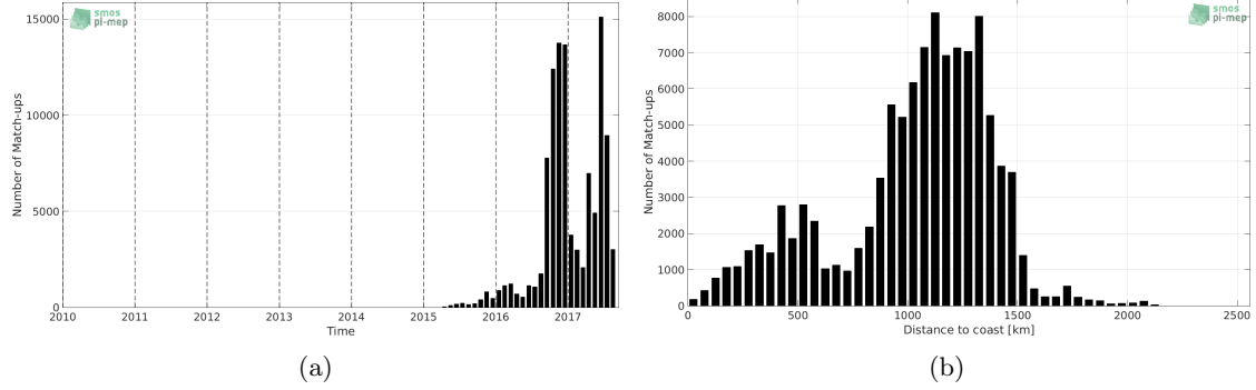
Figure 1: Number of match-ups between Surface drifters and SMAP-L2-RSS-V3-70KM SSS as a function of time (a) and as function of the distance to coast (b) over the Tropical Pacific Ocean Pi-MEP region and for the full satellite product period.
