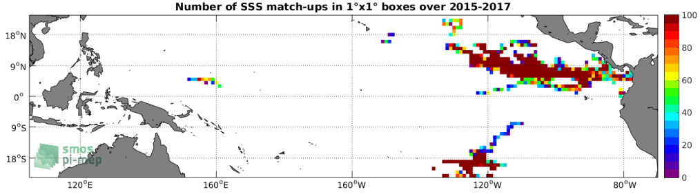
Figure 3: Number of SSS match-ups between Surface drifters SSS and the SMAP-L2-RSS-V3-70KM SSS product for the Tropical Pacific Ocean Pi-MEP region over 1^\circ \times 1^\circ boxes and for the full satellite product period.
