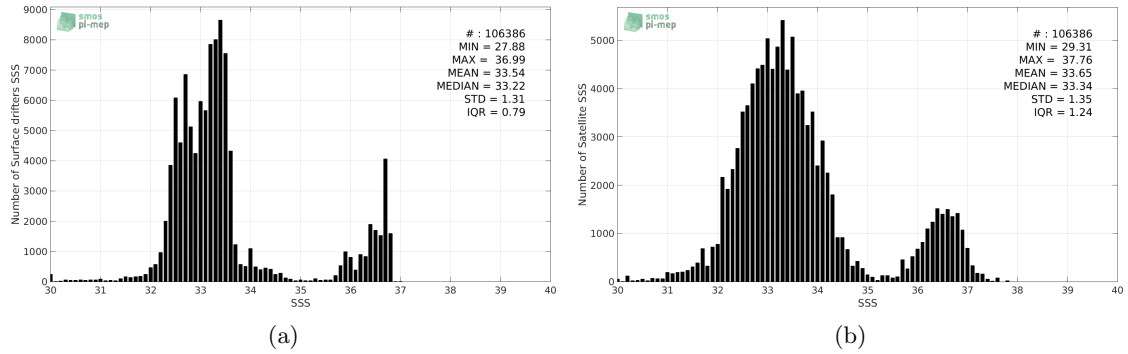
Figure 2: Histograms of SSS from Surface drifters (a) and SMAP-L2-RSS-V3-70KM (b) considering all match-up pairs per bins of 0.1 over the Tropical Pacific Ocean Pi-MEP region and for the full satellite product period.
