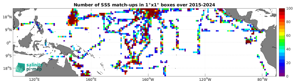
Figure 5: Number of SSS match-ups between TSG (SAMOS) SSS and the SMAP SSS L2 v5.0 (JPL) SSS product for the Tropical Pacific Ocean Pi-MEP region over 1^\circ \times 1^\circ boxes and for the full satellite product period.
