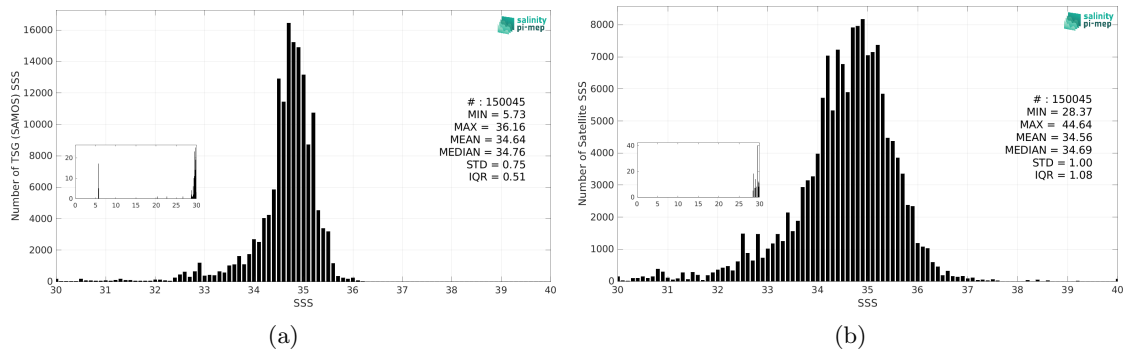
Figure 3: Histograms of SSS from TSG (SAMOS) (a) and SMAP SSS L2 v5.0 (JPL) (b) considering all match-up pairs per bins of 0.1 over the Tropical Pacific Ocean Pi-MEP region and for the full satellite product period.
