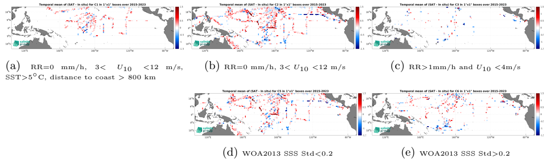
Figure 12: Temporal mean gridded over spatial boxes of size 1^\circ \times 1^\circ of \Delta SSS (SMAP SSS L2 v5.0 (JPL) - TSG (SAMOS)) for 5 different subdatasets corresponding to:RR=0 mm/h, 3 < U_{10} < 12 m/s, SST>5°C, distance to coast > 800 km (a), RR=0 mm/h, 3 < U_{10} < 12 m/s (b), RR>1mm/h and U_{10} < 4 m/s (c), WOA2013 SSS Std<0.2 (d), WOA2013 SSS Std>0.2 (e).
