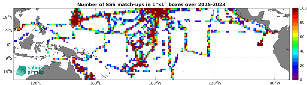
Figure 4: Number of SSS match-ups between TSG (SAMOS) SSS and the SMAP SSS L2 v5.0 (JPL) SSS product for the Tropical Pacific Ocean Pi-MEP region over 1^\circ \times 1^\circ boxes and for the full satellite product period.
