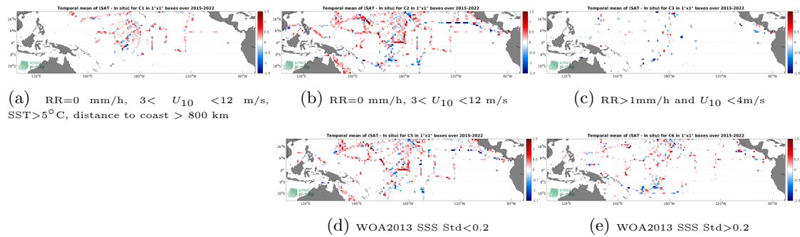
Figure 12: Temporal mean gridded over spatial boxes of size 1^\circ \times 1^\circ of \Delta SSS (SMAP SSS L2 v5.0 (JPL) - TSG (SAMOS)) for 5 different subdatasets corresponding to: RR=0 mm/h, 3 < U_{10} < 12 m/s, SST>5°C, distance to coast > 800 km (a), RR=0 mm/h, 3 < U_{10} < 12 m/s (b), RR>1mm/h and U_{10} < 4 m/s (c), WOA2013 SSS Std<0.2 (d), WOA2013 SSS Std>0.2 (e).
