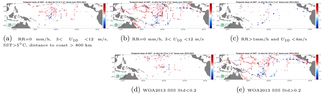
Figure 12: Temporal mean gridded over spatial boxes of size 1^\circ \times 1^\circ of \Delta\text{SSS} (SMAP SSS L2 v5.0 (JPL) - TSG (SAMOS)) for 5 different subdatasets corresponding to:RR=0 mm/h, 3 < U_{10} < 12 m/s, SST>5°C, distance to coast > 800 km (a), RR=0 mm/h, 3 < U_{10} < 12 m/s (b), RR>1mm/h and U_{10} < 4 m/s (c), WOA2013 SSS Std<0.2 (d), WOA2013 SSS Std>0.2 (e).
