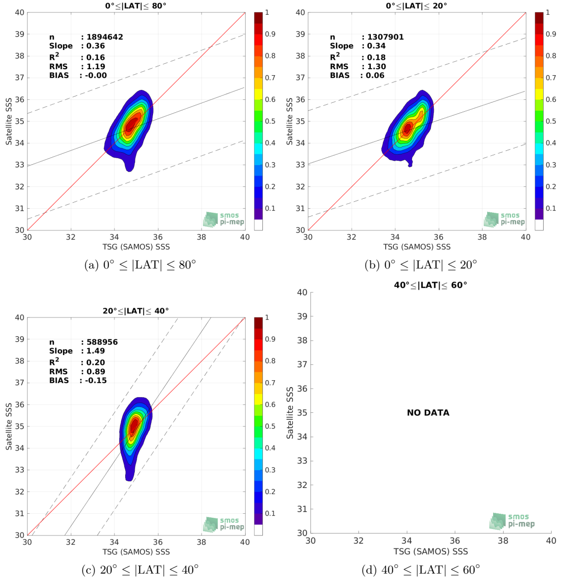
Figure 9: Contour maps of the concentration of SMAP SSS L2 v5.0 (JPL) SSS (y-axis) versus TSG (SAMOS) SSS (x-axis) at match-up pairs for different latitude bands. For each plot, the red line shows x=y . The black thin and dashed lines indicate a linear fit through the data cloud and the \pm 95\% confidence levels, respectively. The number match-up pairs n , the slope and R^2 coefficient of the linear fit, the root mean square (RMS) and the mean bias between satellite and in situ data are indicated for each latitude band in each plots.
