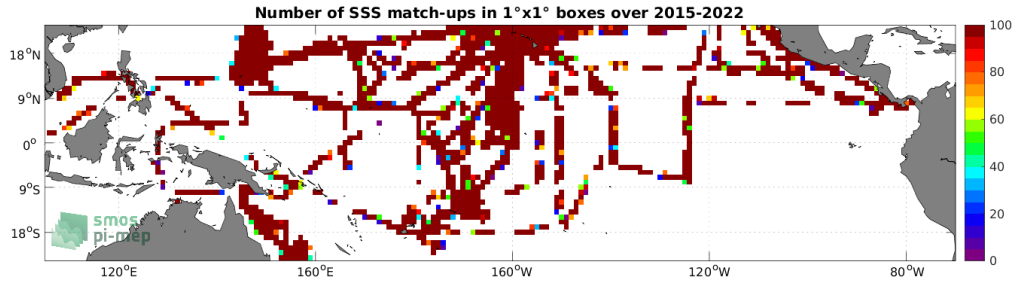
Figure 4: Number of SSS match-ups between TSG (SAMOS) SSS and the SMAP SSS L2 v5.0 (JPL) SSS product for the Tropical Pacific Ocean Pi-MEP region over 1^\circ \times 1^\circ boxes and for the full satellite product period.
