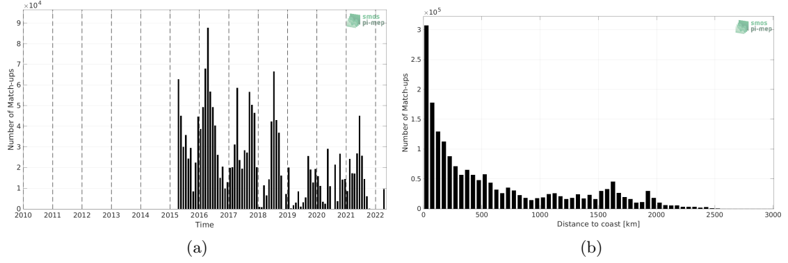
Figure 1: Number of match-ups between TSG (SAMOS) and SMAP SSS L2 v5.0 (JPL) SSS as a function of time (a) and as function of the distance to coast (b) over the Tropical Pacific Ocean Pi-MEP region and for the full satellite product period.
