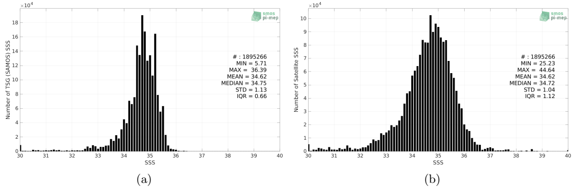
Figure 2: Histograms of SSS from TSG (SAMOS) (a) and SMAP SSS L2 v5.0 (JPL) (b) considering all match-up pairs per bins of 0.1 over the Tropical Pacific Ocean Pi-MEP region and for the full satellite product period.
