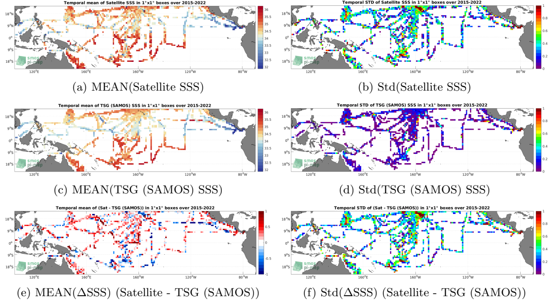
Figure 6: Temporal mean (left) and Std (right) of SSS from SMAP SSS L2 v5.0 (JPL) (top), TSG (SAMOS) (middle), and of \Delta SSS (Satellite - TSG (SAMOS)). Only match-up pairs are used to generate these maps.
