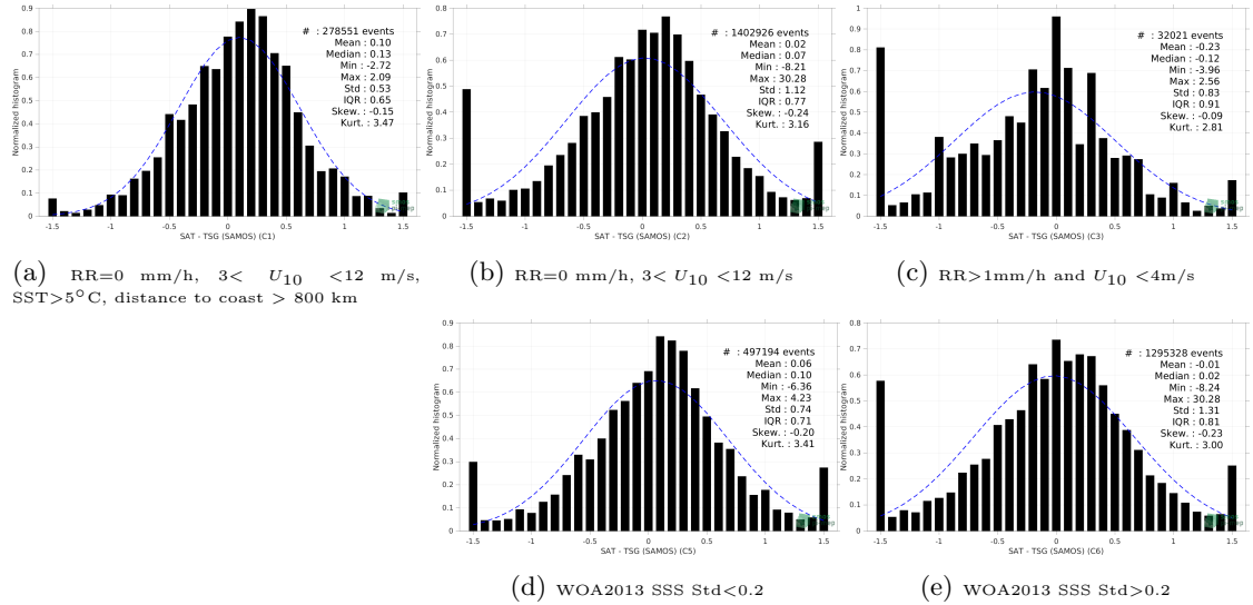
Figure 13: Normalized histogram of \Delta\text{SSS} (SMAP SSS L2 v5.0 (JPL) - TSG (SAMOS)) for 5 different subdatasets corresponding to: RR=0 mm/h, 3 < U_{10} < 12 m/s, SST>5°C, distance to coast > 800 km (a), RR=0 mm/h, 3 < U_{10} < 12 m/s (b), RR>1mm/h and U_{10} < 4 m/s (c), WOA2013 SSS Std<0.2 (d), WOA2013 SSS Std>0.2 (e).
