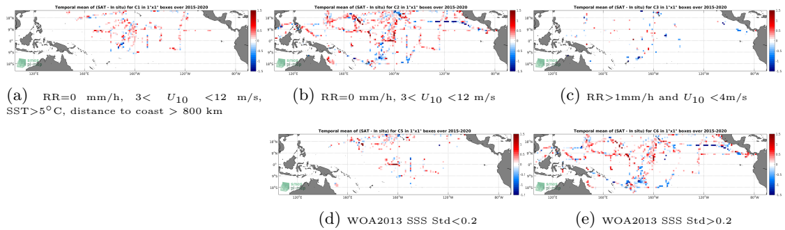
Figure 12: Temporal mean gridded over spatial boxes of size 1°x1° of \Delta SSS (SMAP SSS L2 v5.0 (JPL) - TSG (SAMOS)) for 5 different subdatasets corresponding to:RR=0 mm/h, 3 < U_{10} < 12 m/s, SST>5°C, distance to coast > 800 km (a), RR=0 mm/h, 3 < U_{10} < 12 m/s (b), RR>1mm/h and U_{10} <4m/s (c), WOA2013 SSS Std<0.2 (d), WOA2013 SSS Std>0.2 (e).
